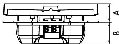
Figure 11: Installation dimensions
