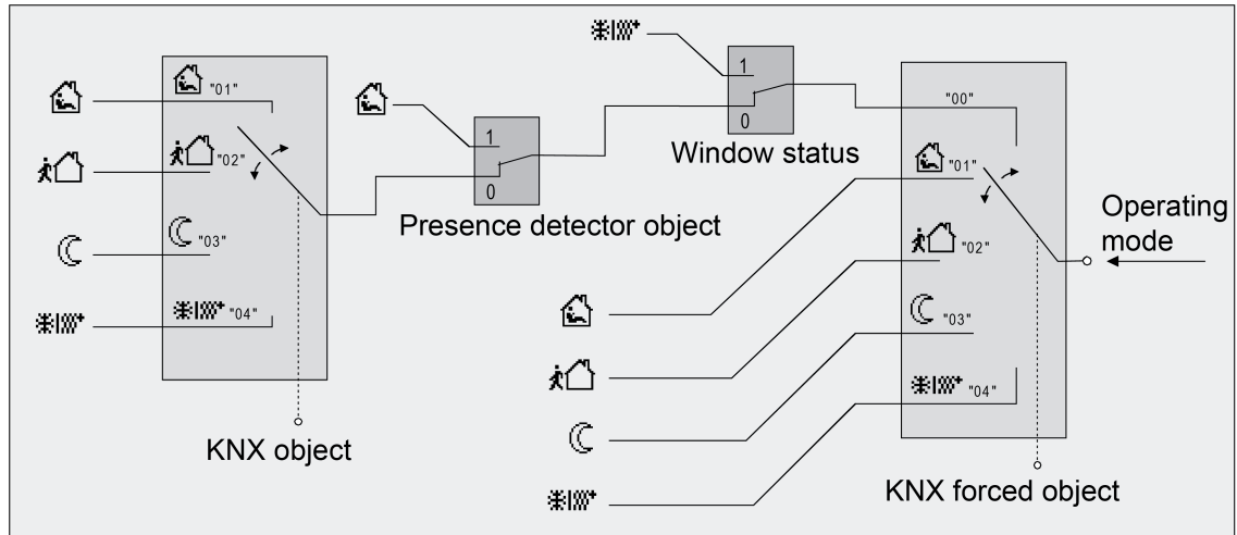
Figure 41: Operating mode change-over through KONNEX object with presence detector
