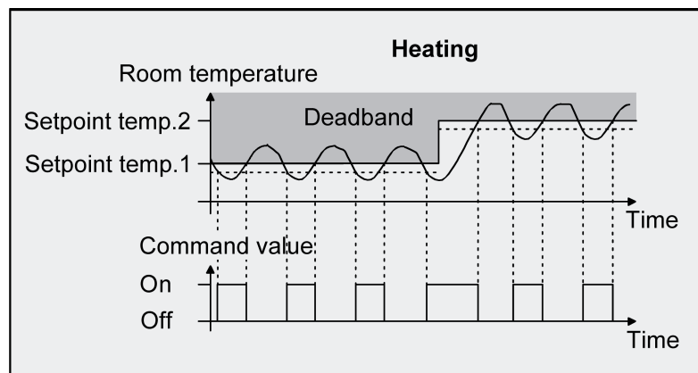
Figure 34: 2-point feedback control for mixed "Heating and cooling" mode with active heating mode.
