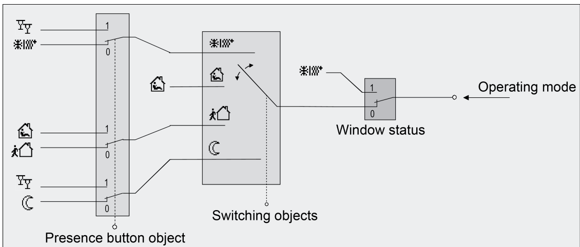
Figure 38: Operating mode change-over through 4 x 1-bit objects with presence button
