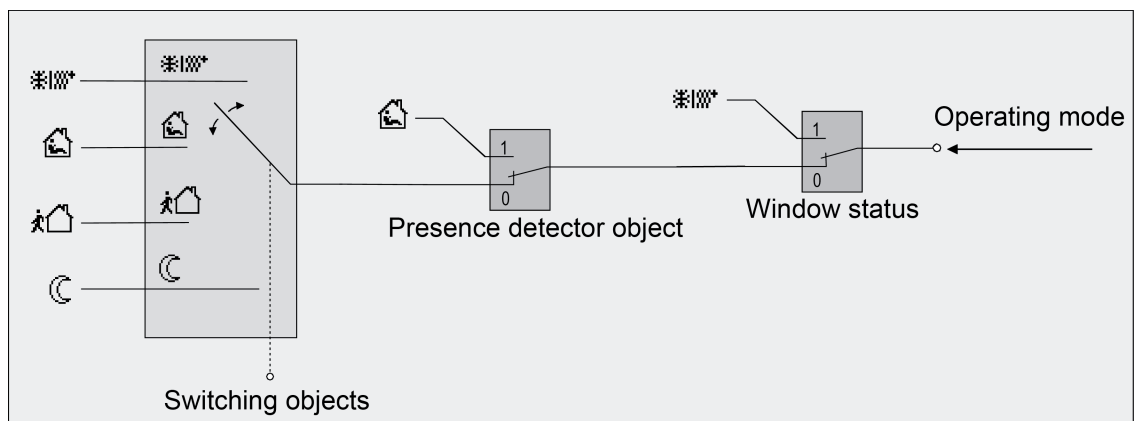
Figure 39: Operating mode change-over through 4 x 1-bit objects with presence detector
