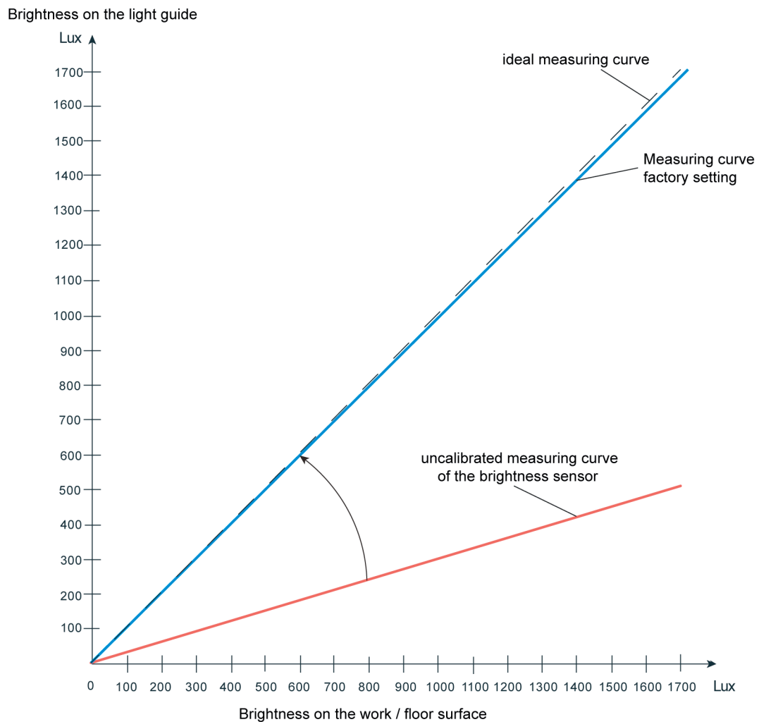
Figure 18: Determining the brightness on the work / floor surface during factory setting Reflection coefficient 0.3 corresponds to surface finish (grey desktop)
