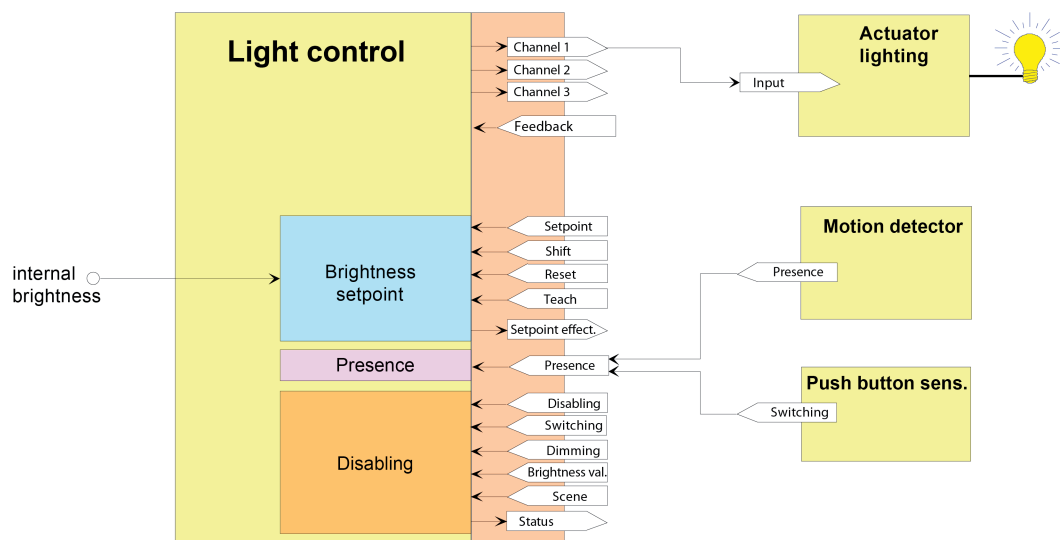
Figure 45: Application example for light control in autonomous operation
