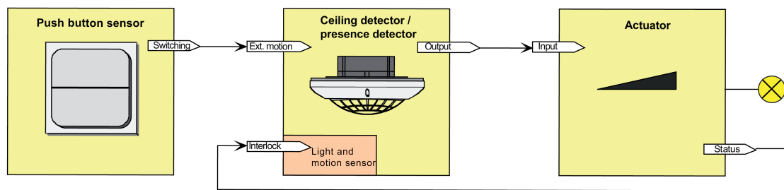
Figure 30: Application example of single device with external motion detection
