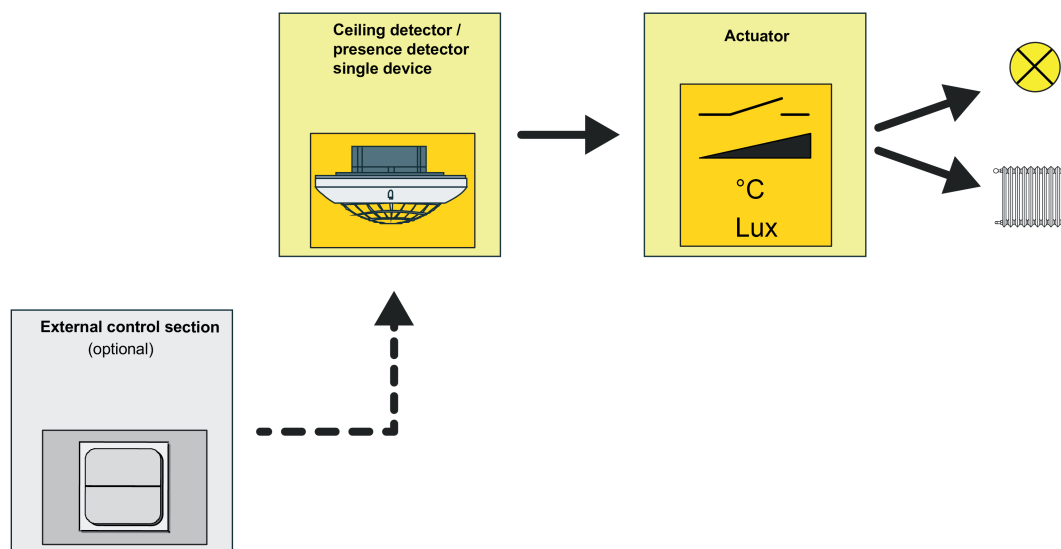
Figure 26: Application type "single device"
