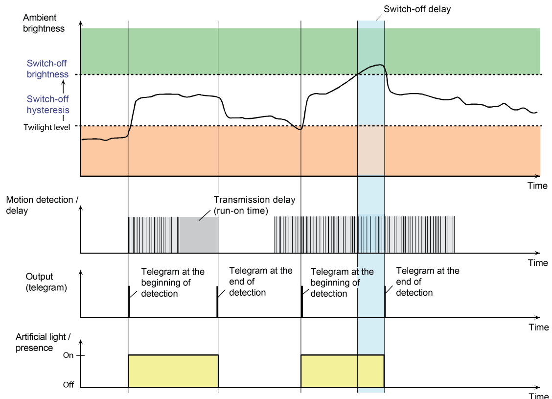
Figure 23: Brightness and motion evaluation with the presence detector
