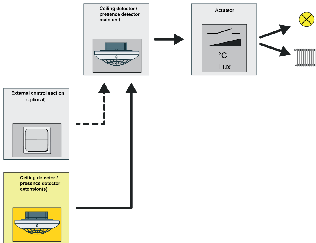
Figure 28: Application type "Extension"
