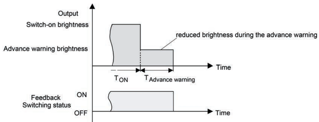
Figure 44: The pre-warning function of the staircase function without soft OFF function
