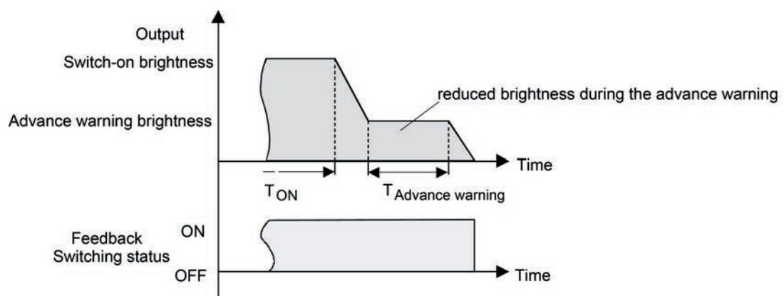
Figure 45: The pre-warning function of the staircase function with soft OFF function (as an example with minimum brightness = 0 %)
