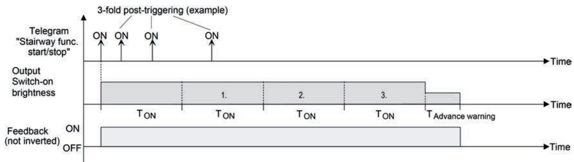
Figure 48: Time extension of the staircase function
