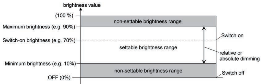
Figure 34: Example of a brightness range with switch-on brightness
