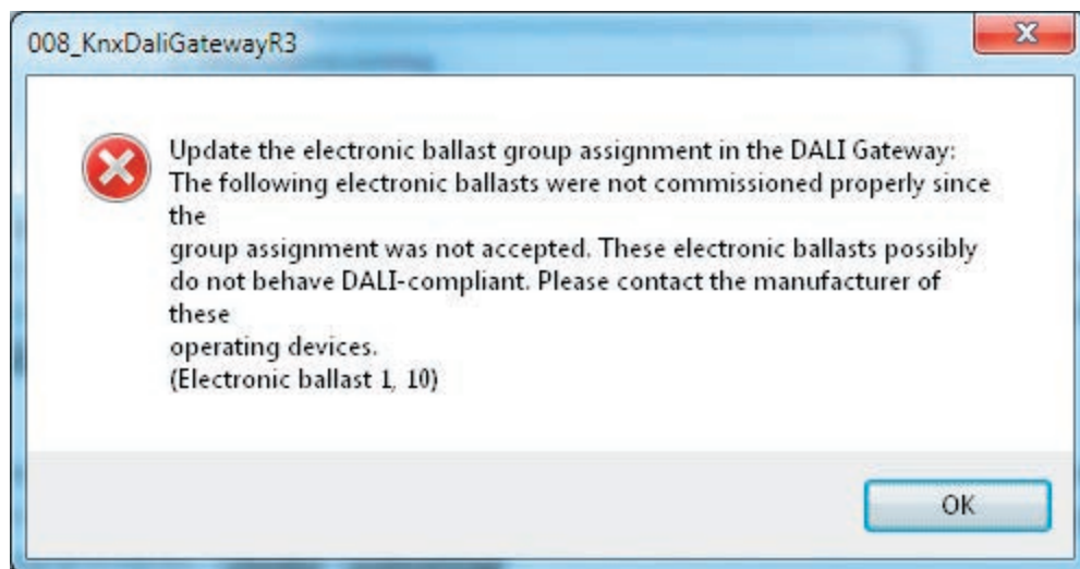
Figure 73: Error message of DALI group assignment
