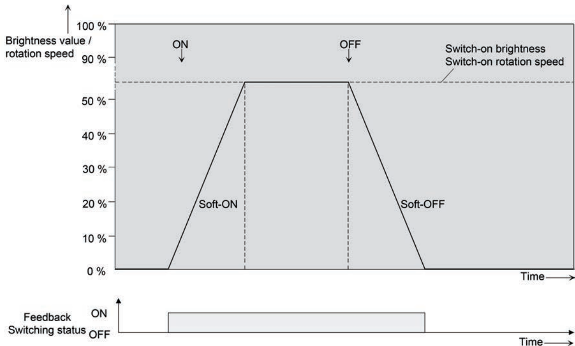
Figure 39: Dimming behaviour of the soft ON/OFF functions with minimum brightness > 0%
