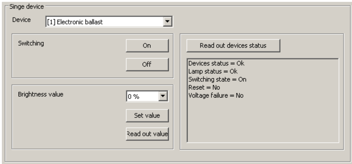
Figure 75: Device-orientated DALI test environment
