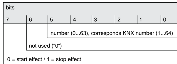
Figure 55: Structure of the object value for the effect extension
