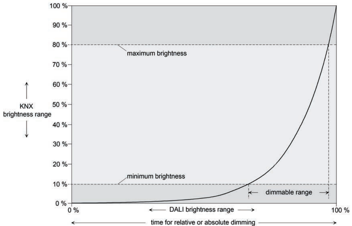
Figure 37: Dimming characteristic for relative or absolute dimming as an example with minimum brightness and maximum brightness
