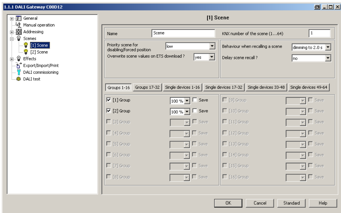
Figure 50: Configuration page of a scene as an example with two created effect scenes and two DALI groups
