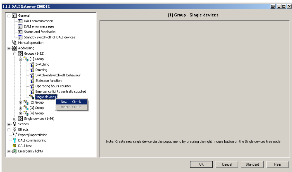
Figure 71: Assigning an electronic ballast to a group - offline commissioning
