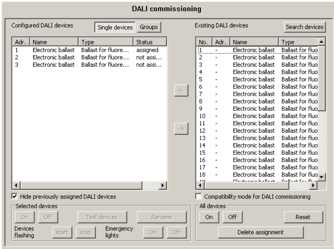
Figure 67: Operating device assigned to a programmed single device
