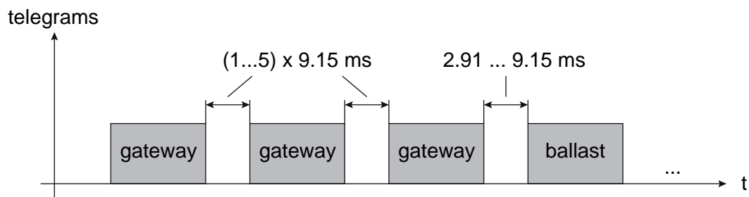
Figure 29: Pause times between DALI telegrams
