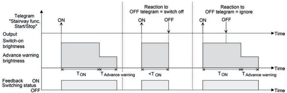
Figure 42: Switch-off behaviour of the staircase function without soft functions
