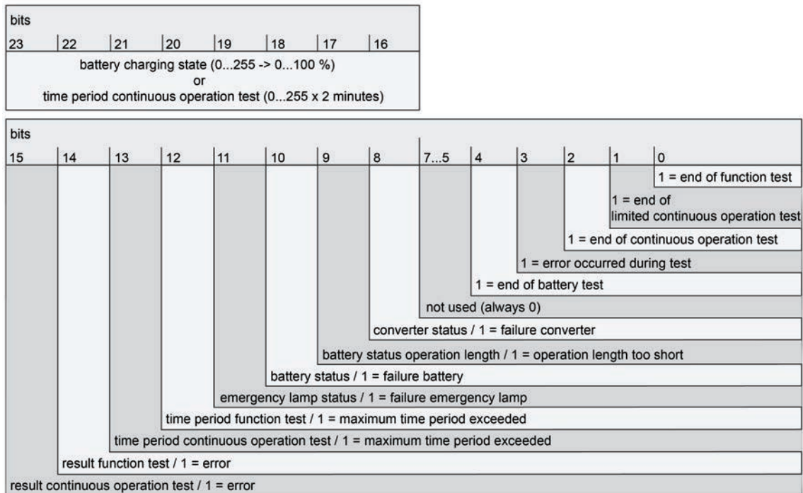
Figure 58: Structure of the 3-byte object "Feedback, emergency operation test"
