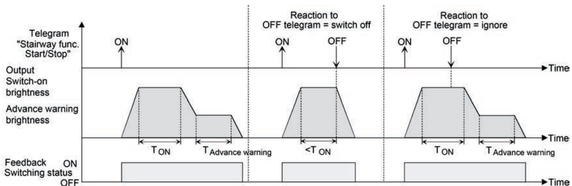
Figure 43: Switch-off behaviour of the staircase function with soft functions (as an example with minimum brightness = 0 %)
