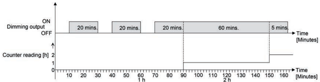
Figure 49: Function of the operating hours counter (using the example of an up-counter)
