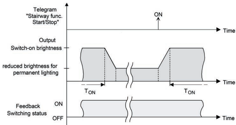
Figure 47: The continuous lighting of the staircase function with soft OFF functions
