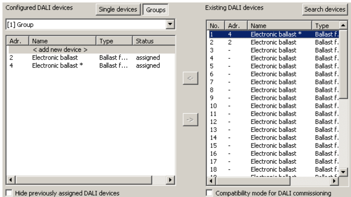
Figure 66: Operating device assigned to a group Here: Electronic ballast with the address 3 is assigned to multiple groups.
