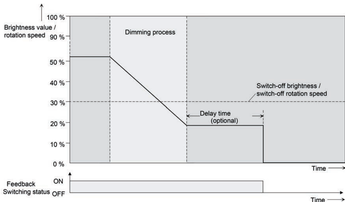
Figure 38: Dimming and switching behaviour of the automatic switch-off function
