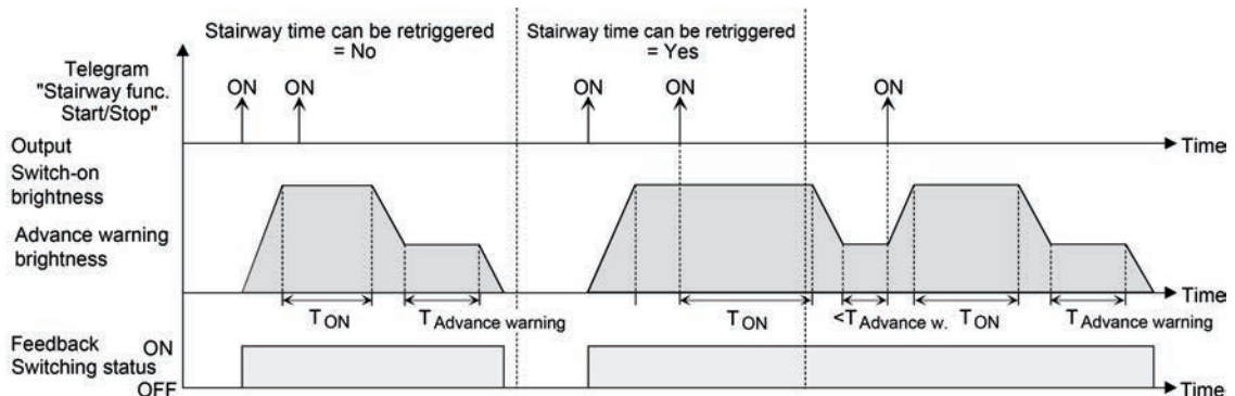
Figure 41: Switch-on behaviour of the staircase function with soft functions (as an example with minimum brightness = 0 %)
