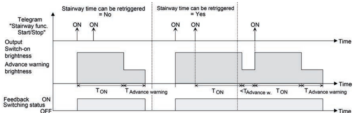
Figure 40: Switch-on behaviour of the staircase function without soft functions
