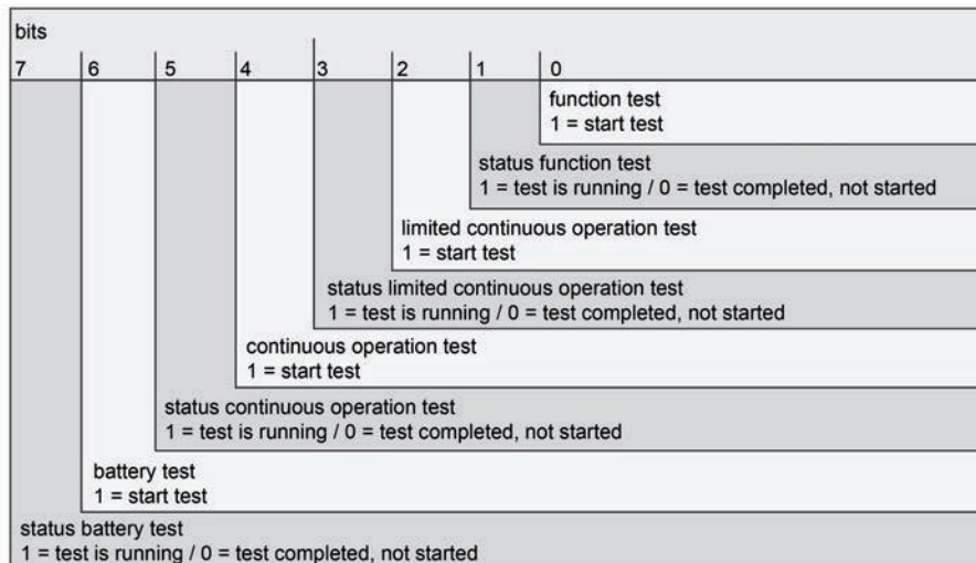
Figure 57: Structure of the 1-byte object "Emergency operation test start / status"
