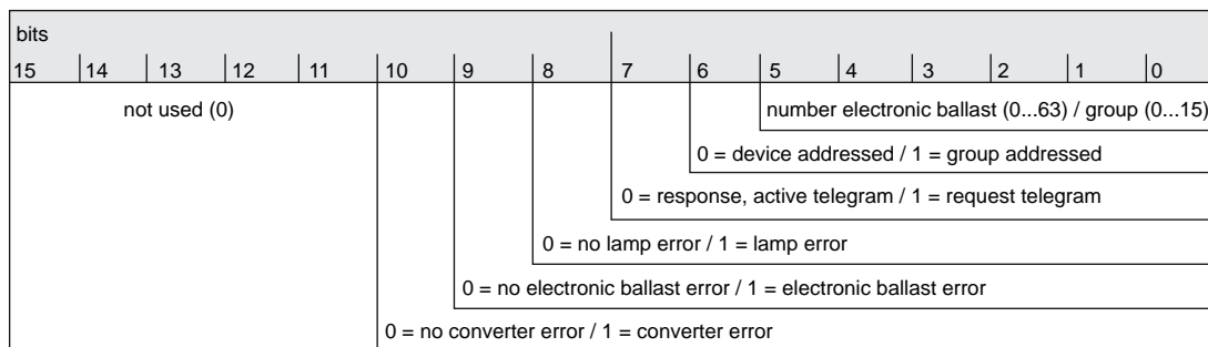
Figure 31: Telegram structure, 2-byte KNX error status
