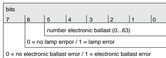
Figure 30: Telegram structure, 1-byte error status
