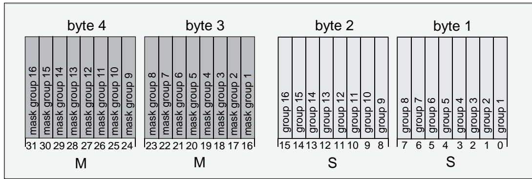
Figure 32: Structure of the objects of the collective feedback, using the example of the object for Groups 1-16
