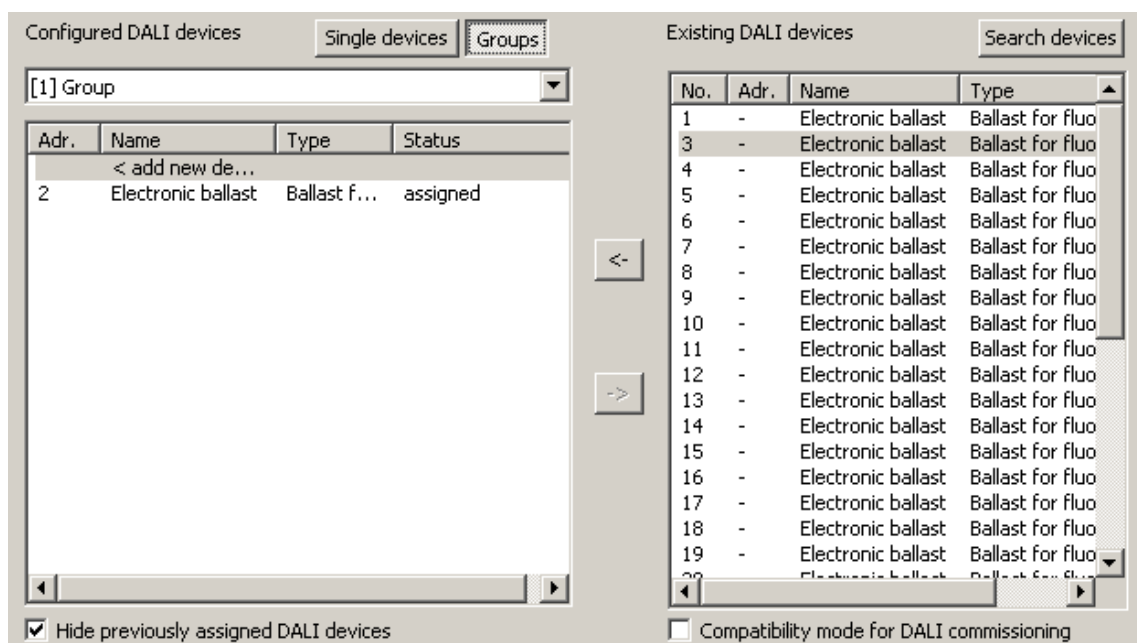
Figure 65: Operating device assigned to a group
