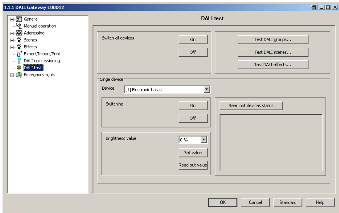
Figure 74: DALI test environment in the ETS3 plug-in
