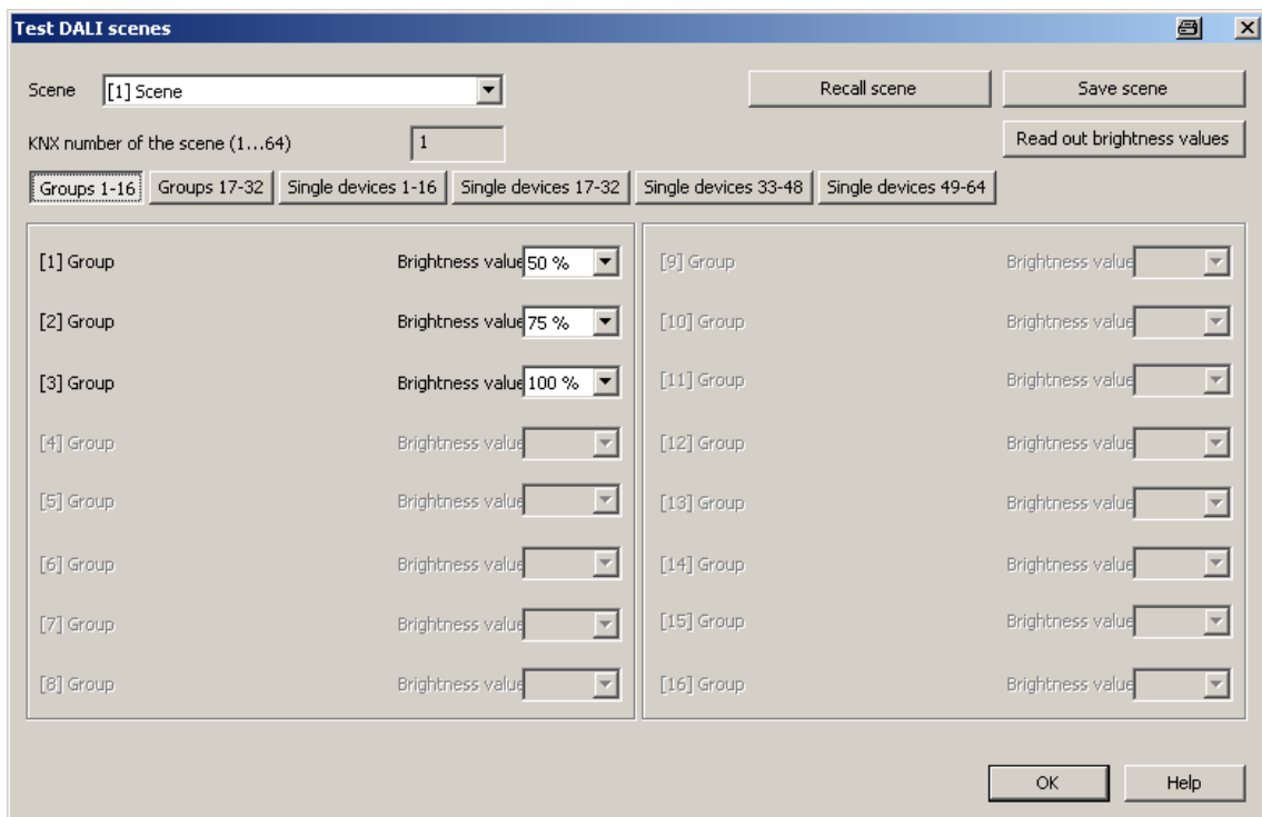
Figure 78: Scene-orientated DALI test environment (as an example with Scene 1 with three created groups)
