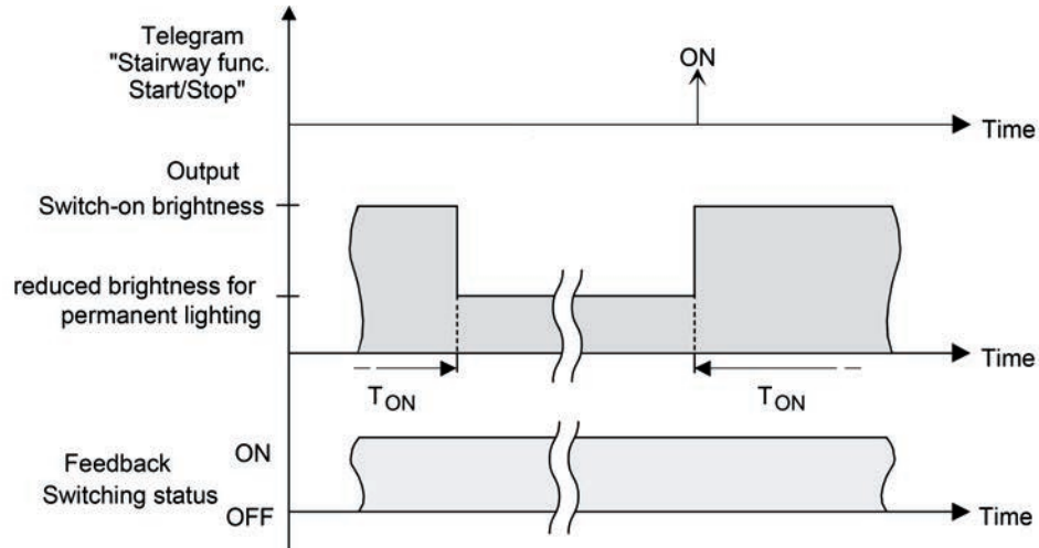
Figure 46: The continuous lighting of the staircase function without soft functions
