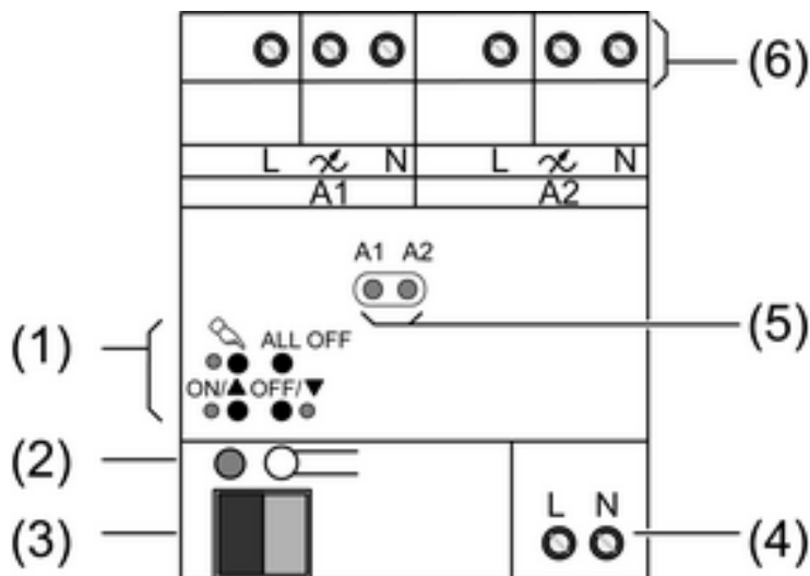
Figure 1: View of dimmer actuator 2gang
