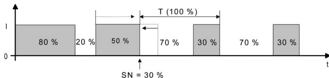
Figure 19: Command value change, e.g. from 80 % to 30 % during the opening phase of the valve (opening phase too long)
