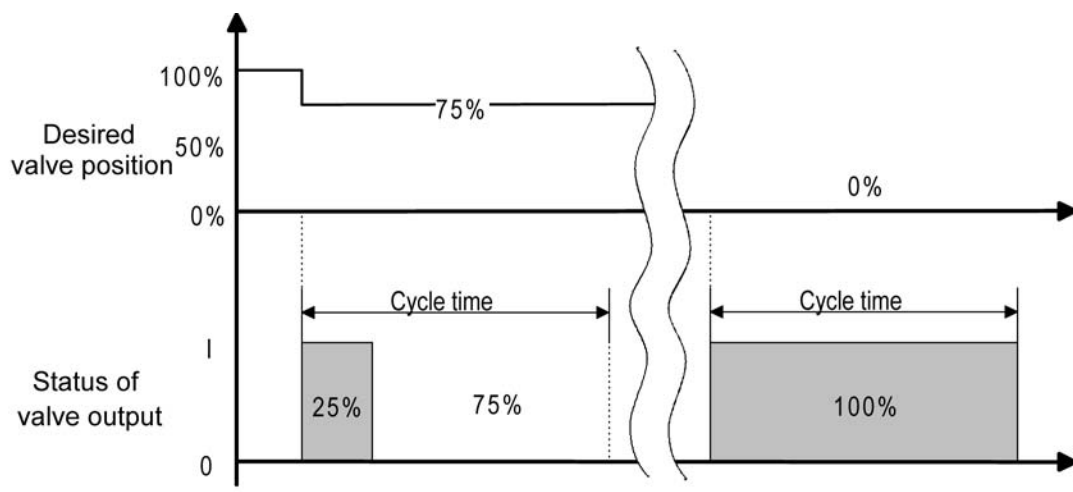
Figure 13: Conversion of a constant valve setpoint position to an output signal with deenergised, opened valve drives (example)
