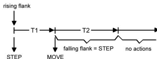
Figure 6: Operation concept "short – long – short"
