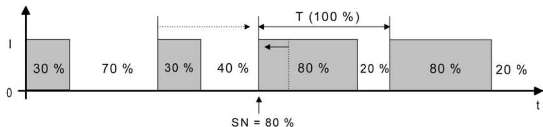
Figure 22: Command value change, e.g. from 30 % to 80 % during the closing phase of the valve (closing phase too long)
