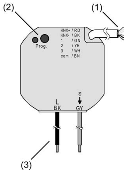
Figure 1: Device components
