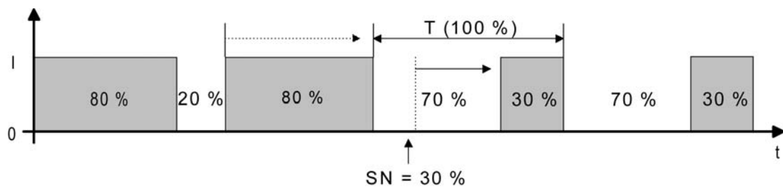
Figure 18: Command value change, e.g. from 80 % to 30 % during the closing phase of the valve
