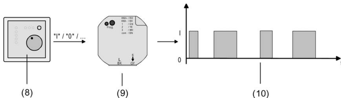
Figure 14: Command value principle for switching command value
