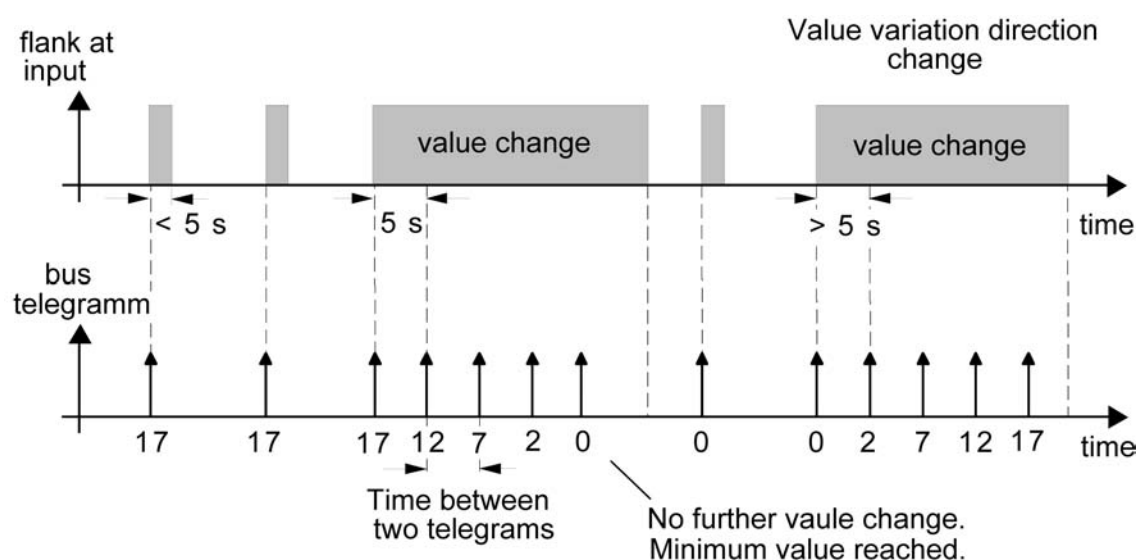
Figure 8: Example to change the value for dimming value encoder
