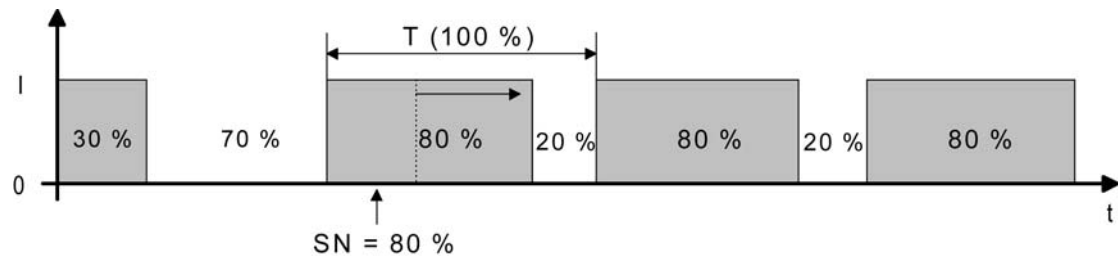
Figure 20: Command value change, e.g. from 30 % to 80 % during the opening phase of the valve
