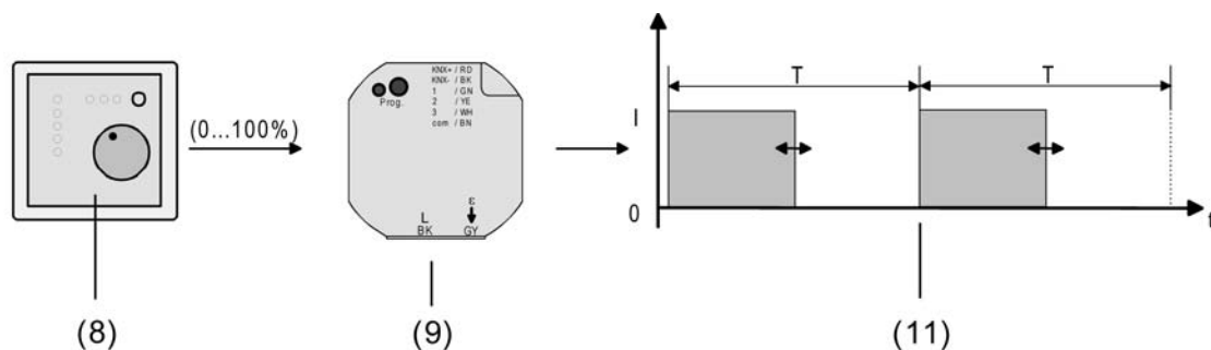
Figure 15: Command value principle for constant command value
