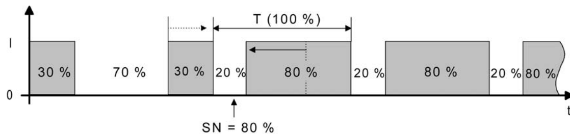
Figure 21: Command value change, e.g. from 30 % to 80 % during the closing phase of the valve
