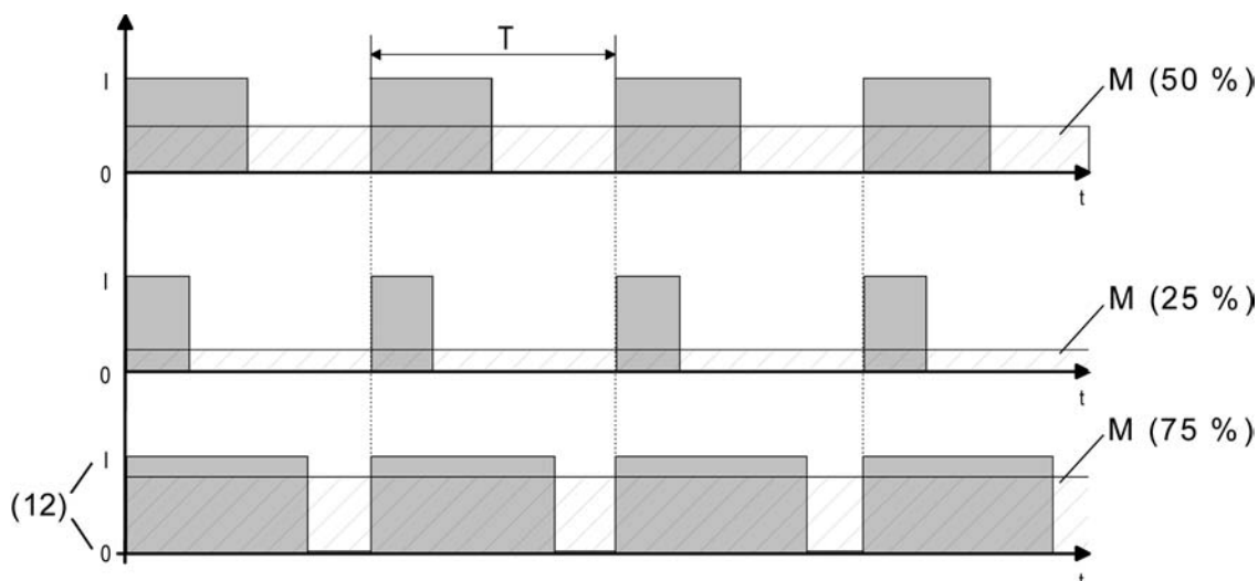
Figure 16: Pulse width modulation of a valve output signal
