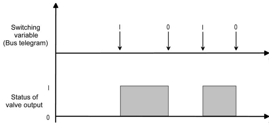
Figure 10: Conversion of a switching command value to an output signal with deenergised, closed valve drives (example)
