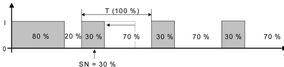
Figure 17: Command value change, e.g. from 80 % to 30 % during the opening phase of the valve
