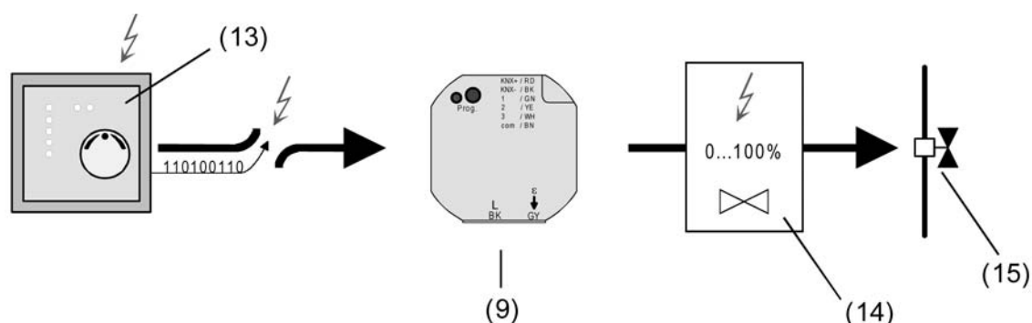
Figure 25: Principle of cyclical command value monitoring in the event of a fault (e.g. open circuit)
