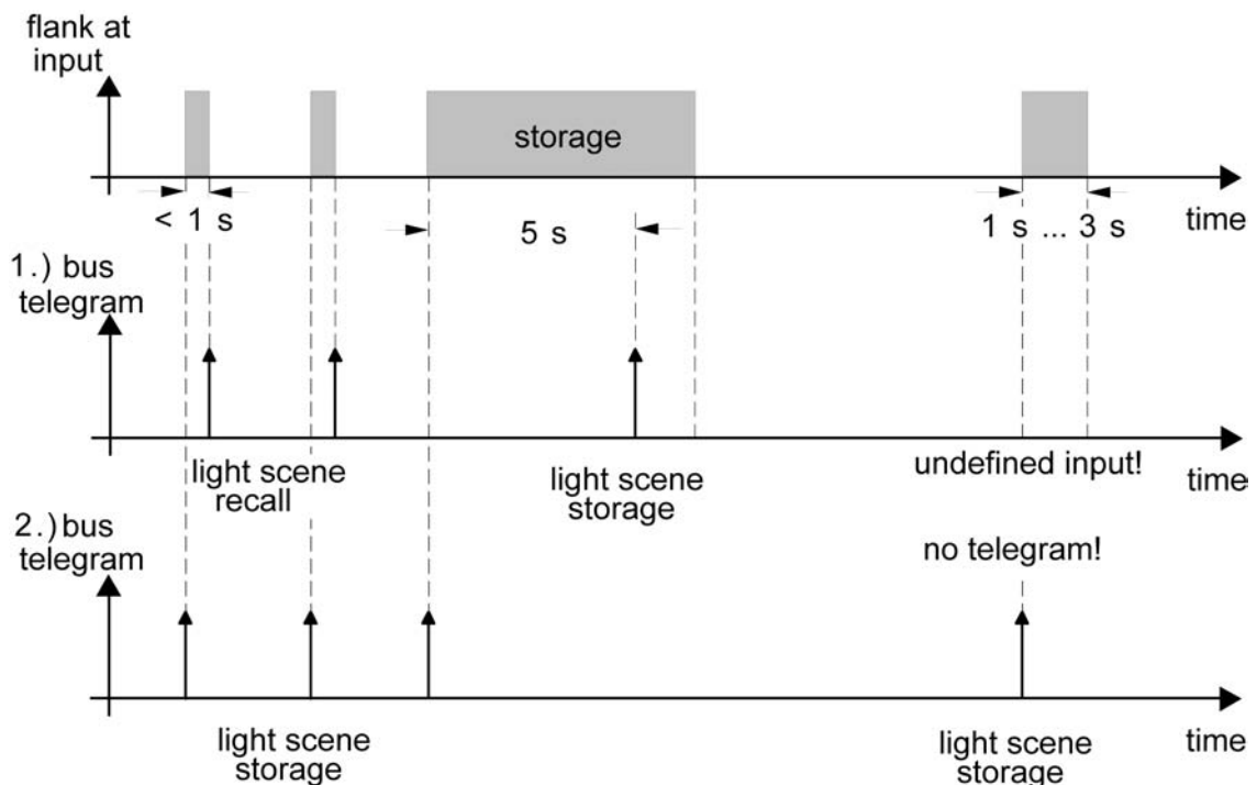
Figure 9: Example of scene storage
