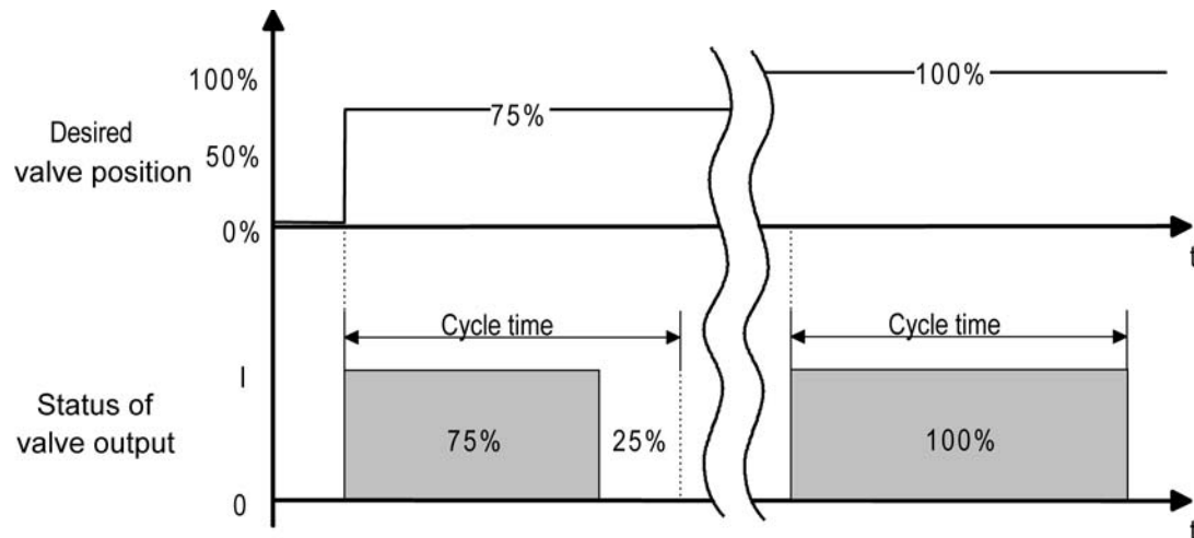
Figure 11: Conversion of a constant valve setpoint position to an output signal with deenergised, closed valve drives (example)
