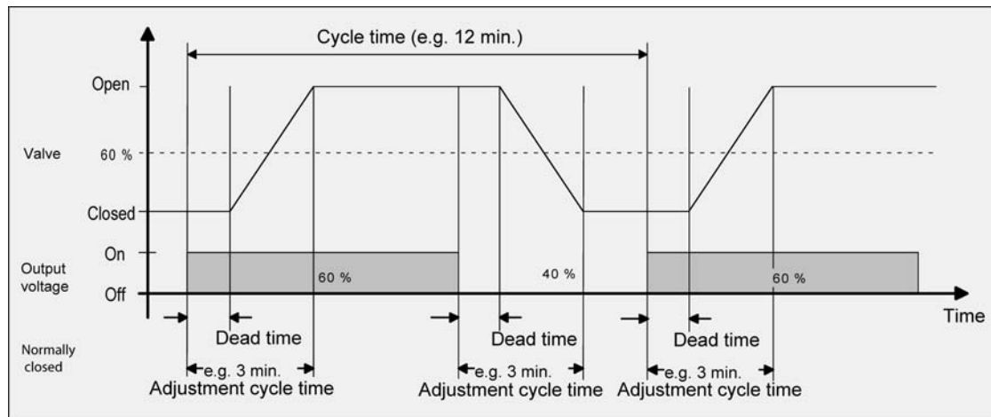
Figure 23: Ideal course of the valve stroke for a command value of approx. 60 % of a deenergised, closed valve
