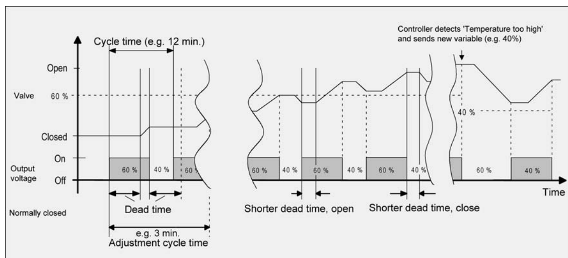
Figure 24: Ideal course of the valve stroke for a command value of approx. 60 % at first of a deenergised, closed valve
