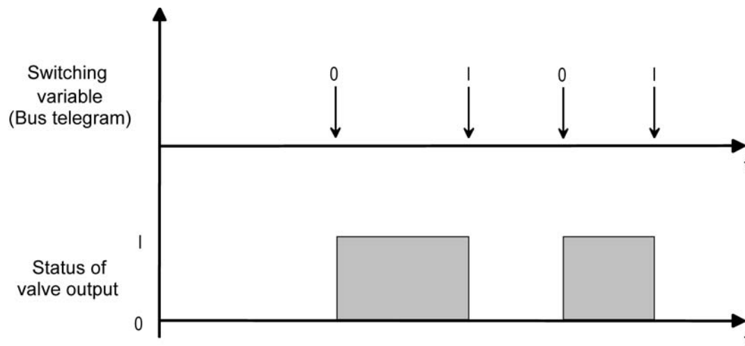
Figure 12: Conversion of a switching command value to an output signal with deenergised, opened valve drives (example)
