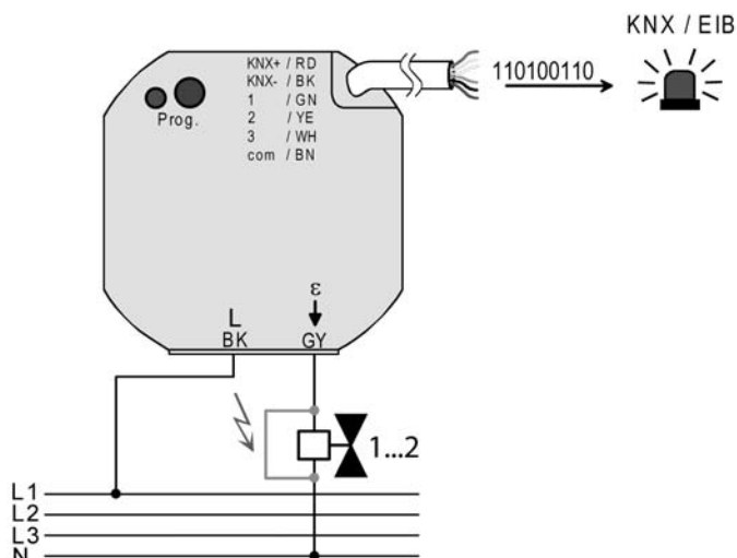
Figure 26: Short-circuit and overload detection in case of fault in valve output or valve drive
