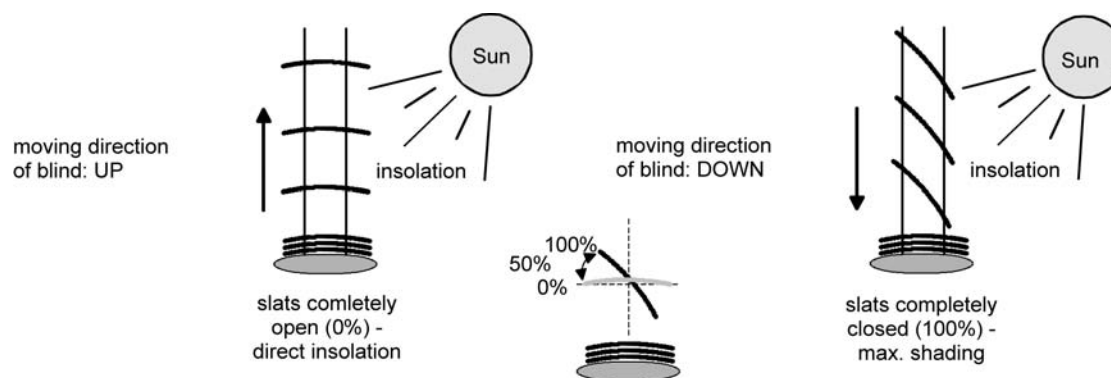
Figure 13: Type 2 - Slatted Venetian blinds with oblique and horizontal slat position
