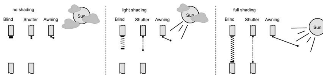
Figure 19: Sun protection principles (example)
