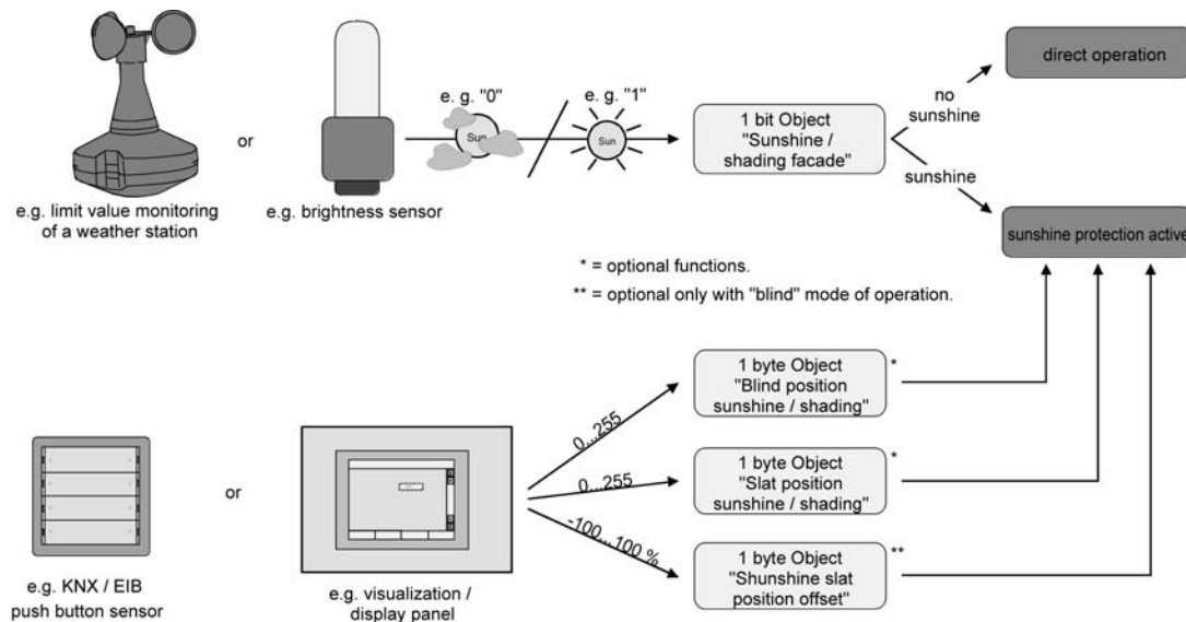
Figure 20: Schematic diagram illustrating the simple sun protection configuration
