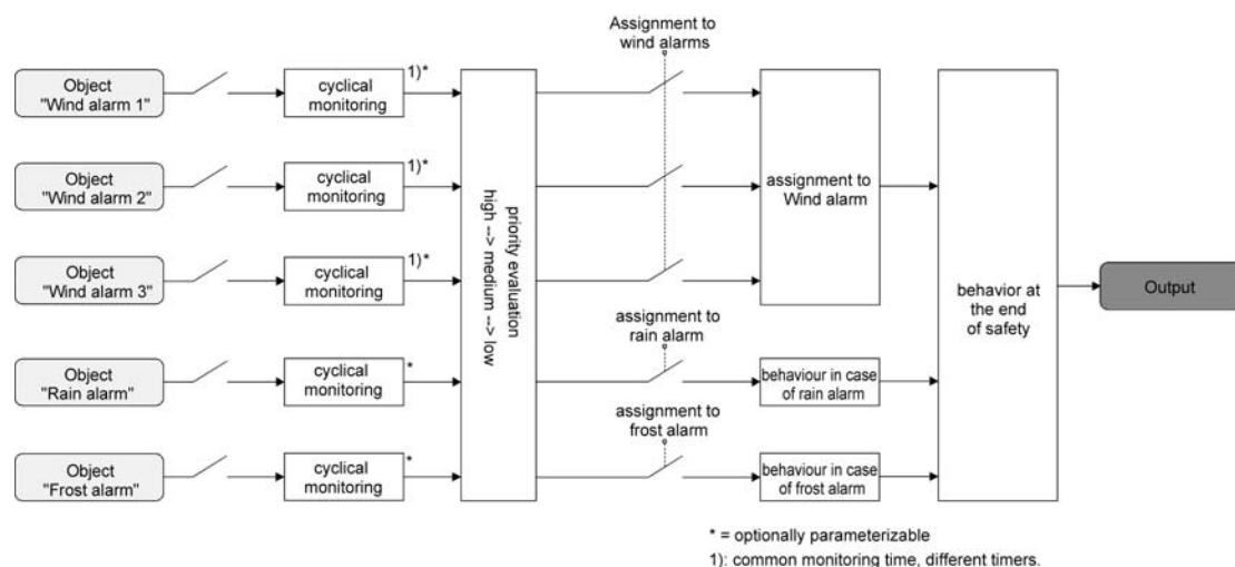
Figure 18: Function diagram of the safety function
