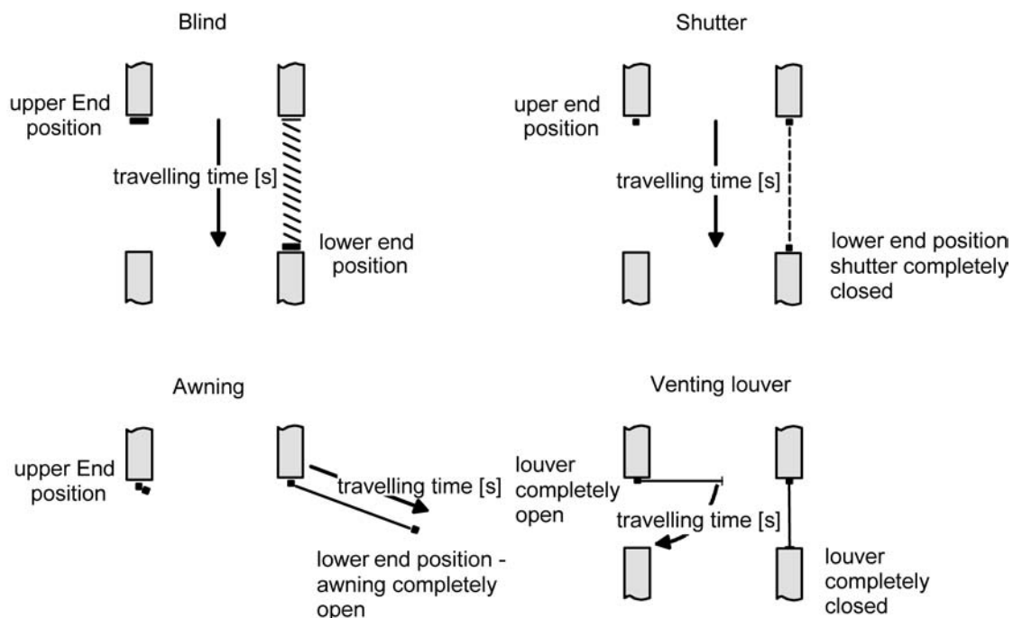
Figure 11: Determining the movement time according to the drive type
