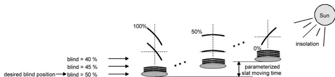
Figure 15: Example of slat positioning affecting the position of the Venetian blind (typical of slat type 1; analogous reaction for type 2)
