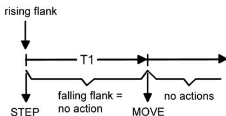
Figure 8: Operation concept "long – short"
