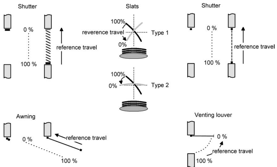
Figure 17: Reference movement
