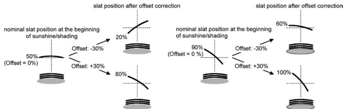
Figure 24: Functional principle of slat offset (example showing slat type 1 / slat type 2 identical)
