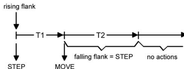
Figure 7: Operation concept "short - long - short"
