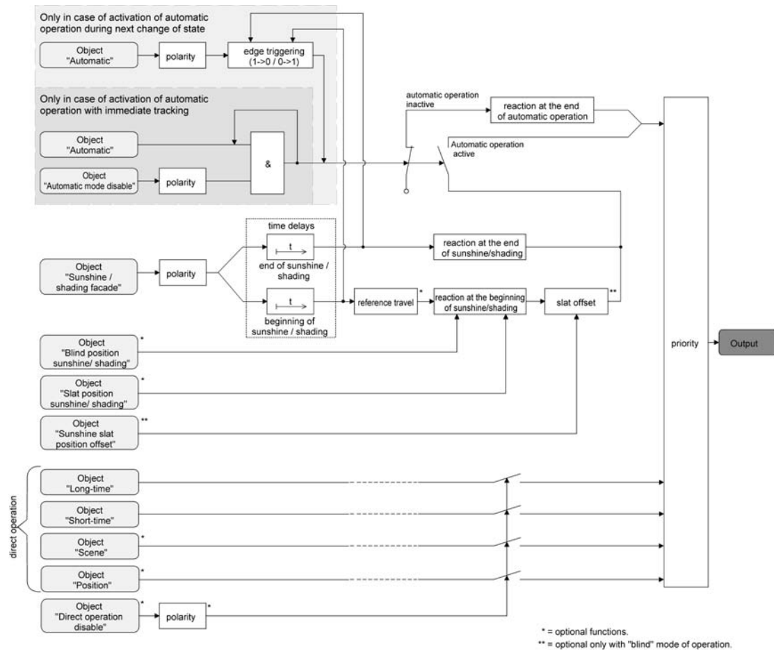
Figure 23: Function diagram illustrating the extended sun protection
