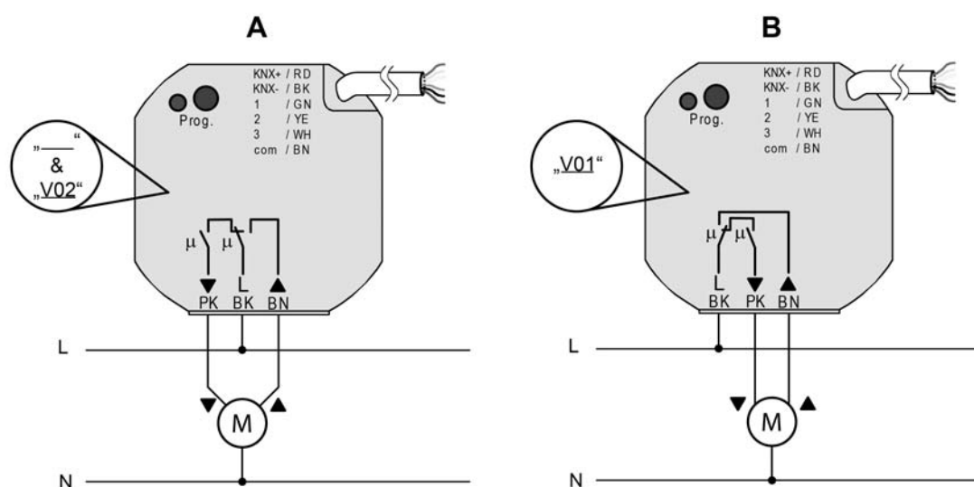
Figure 4: Connection of the mains voltage and the load (depending upon the version labelling)
