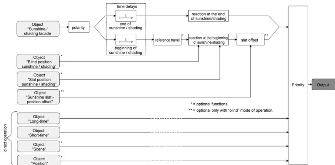
Figure 21: Function diagram illustrating the simple sun protection
