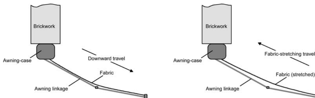
Figure 32: Fabric stretching in an awning
