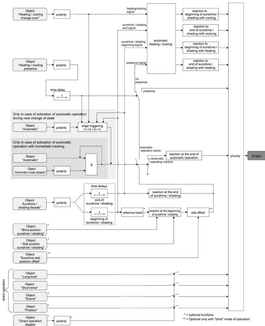
Figure 31: Schematic function diagram of automatic heating/cooling
