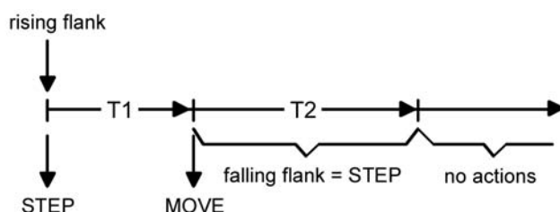
Figure 6: Operating concept "Short - long - short" when inputs 1 and 2 have an internal impact
