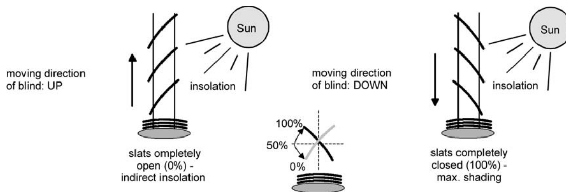
Figure 12: Type 1 - Slatted Venetian blinds with oblique slat position in both travel directions
