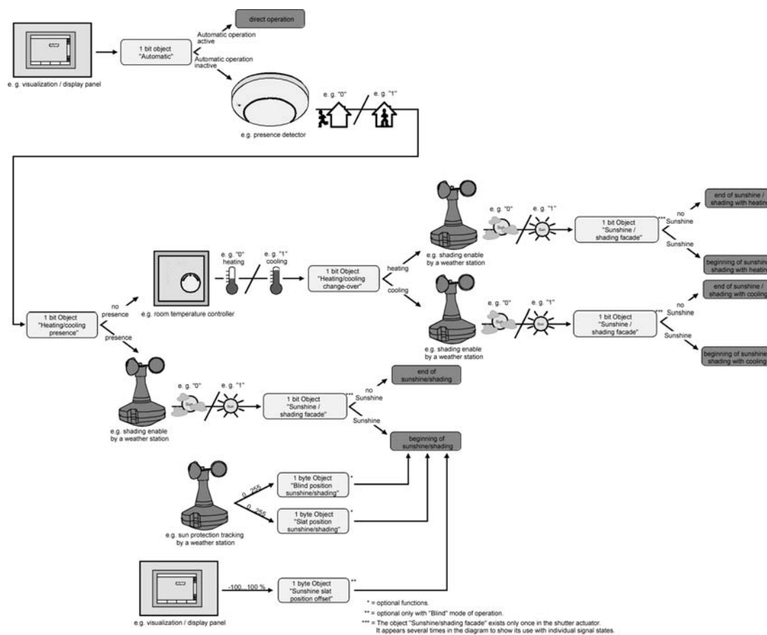
Figure 30: Schematic diagram of automatic heating/cooling (for reasons of simplicity shown without disabling functions of the automatic or direct operation)
