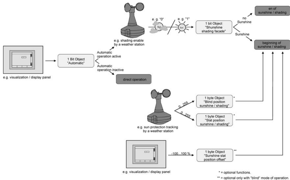
Figure 22: Schematic diagram illustrating the extended sun protection configuration (for reasons of simplicity without disabling functions)
