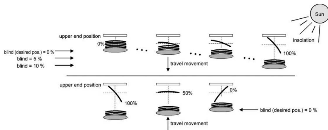
Figure 16: Example of slat positioning with the Venetian blind in upper end position (typical of slat type 1)
