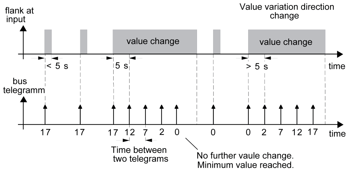
Figure 9: Example to change the value for dimming value encoder
