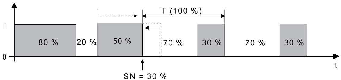
Figure 42: Command value change, e.g. from 80 % to 30 % during the opening phase of the valve (opening phase too long)
