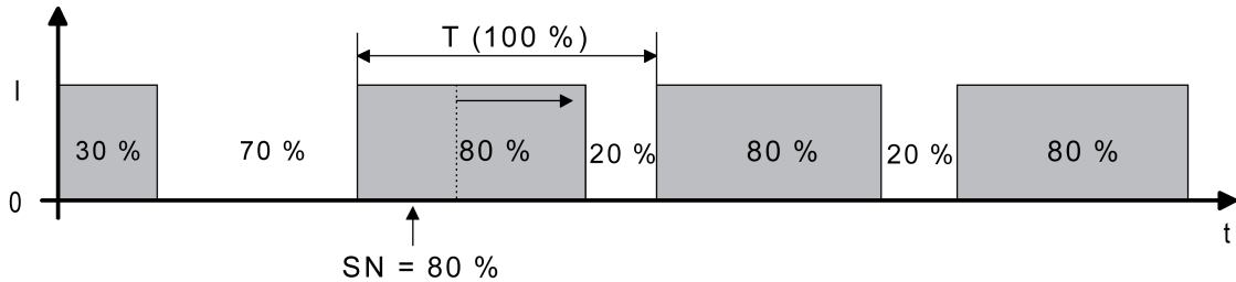
Figure 43: Command value change, e.g. from 30 % to 80 % during the opening phase of the valve
