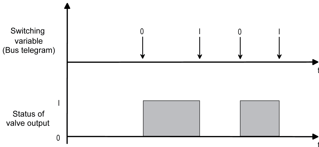
Figure 35: Conversion of a switching command value to an output signal with deenergised, opened valve drives (example)
