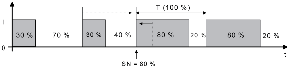
Figure 45: Command value change, e.g. from 30 % to 80 % during the closing phase of the valve (closing phase too long)
