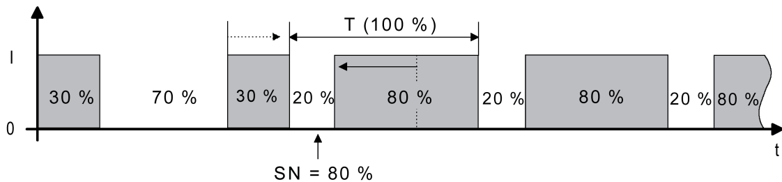
Figure 44: Command value change, e.g. from 30 % to 80 % during the closing phase of the valve
