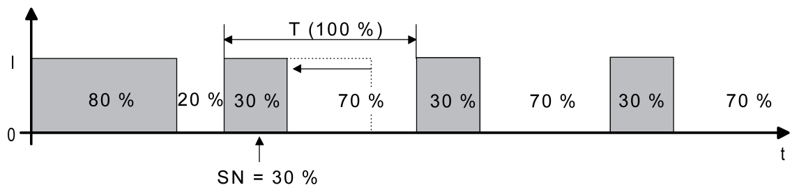
Figure 40: Command value change, e.g. from 80 % to 30 % during the opening phase of the valve
