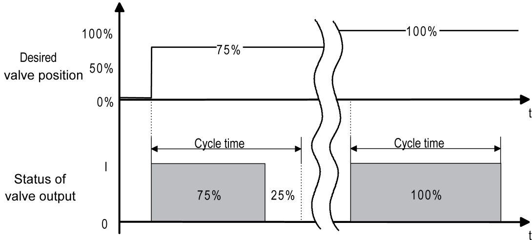
Figure 34: Conversion of a constant valve setpoint position to an output signal with deenergised, closed valve drives (example)
