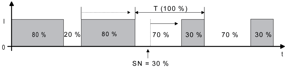
Figure 41: Command value change, e.g. from 80 % to 30 % during the closing phase of the valve
