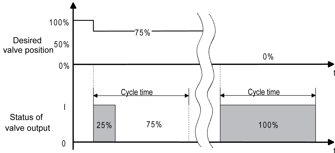
Figure 36: Conversion of a constant valve setpoint position to an output signal with deenergised, opened valve drives (example)
