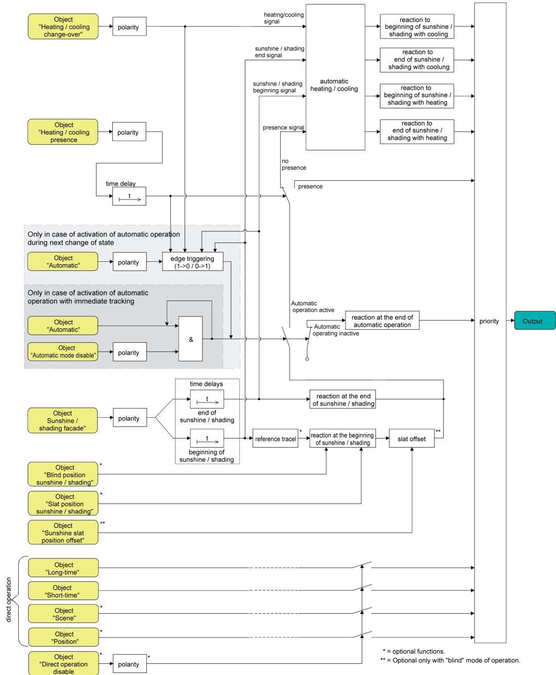
Figure 31: Schematic function diagram of automatic heating/cooling
