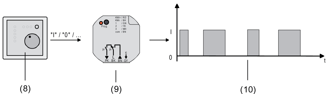
Figure 37: Command value principle for switching command value
