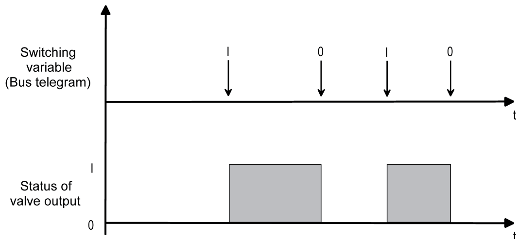
Figure 33: Conversion of a switching command value to an output signal with deenergised, closed valve drives (example)
