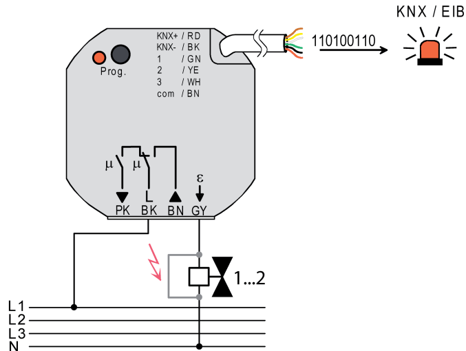
Figure 49: Short-circuit and overload detection in case of fault in valve output or valve drive
