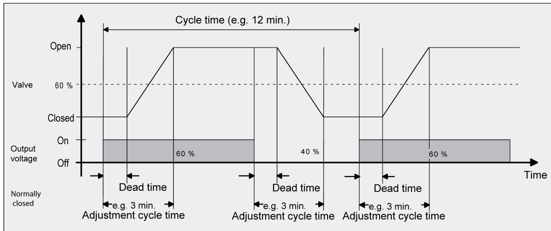
Figure 46: Ideal course of the valve stroke for a command value of approx. 60 % of a deenergised, closed valve
