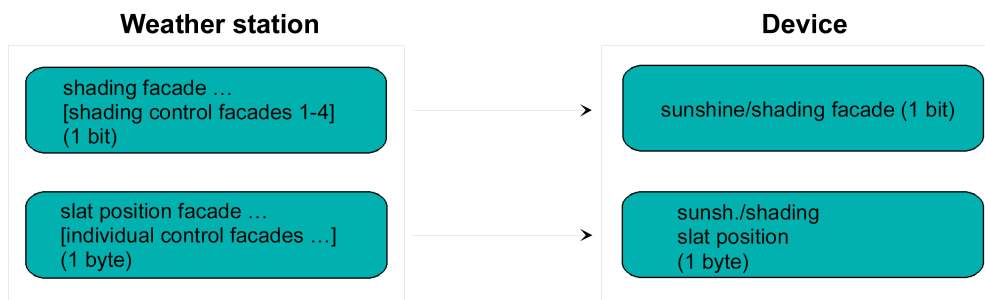
Figure 27: Programming of the communication objects for application example III
