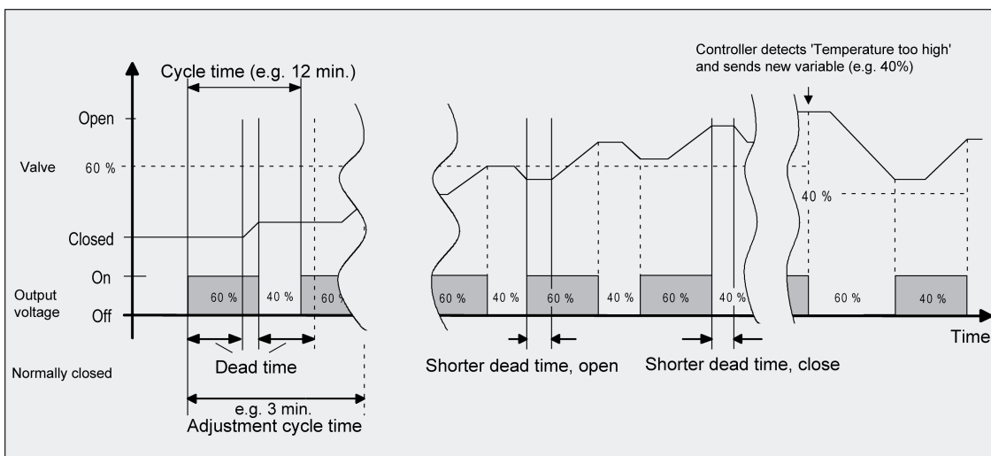
Figure 47: Ideal course of the valve stroke for a command value of approx. 60 % at first of a deenergised, closed valve
