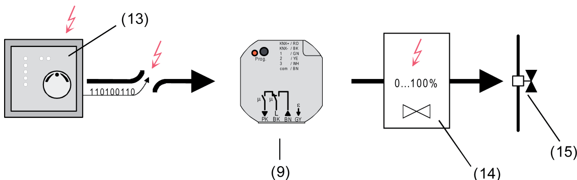
Figure 48: Principle of cyclical command value monitoring in the event of a fault (e.g. open circuit)
