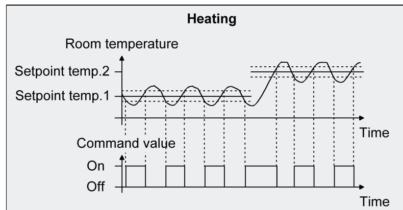
Figure 33: 2-point feedback control for the single "Heating" operating mode
