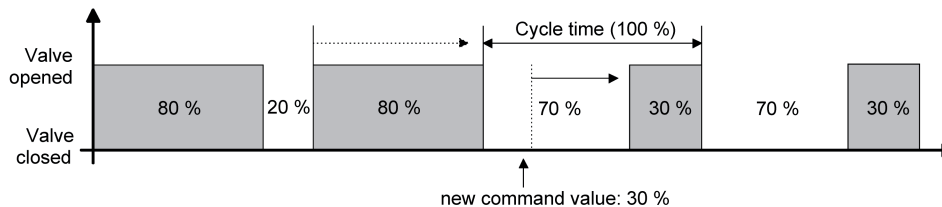
Figure 12: Example of a command value change 80 % -> 30 % during the closing phase of the valve
