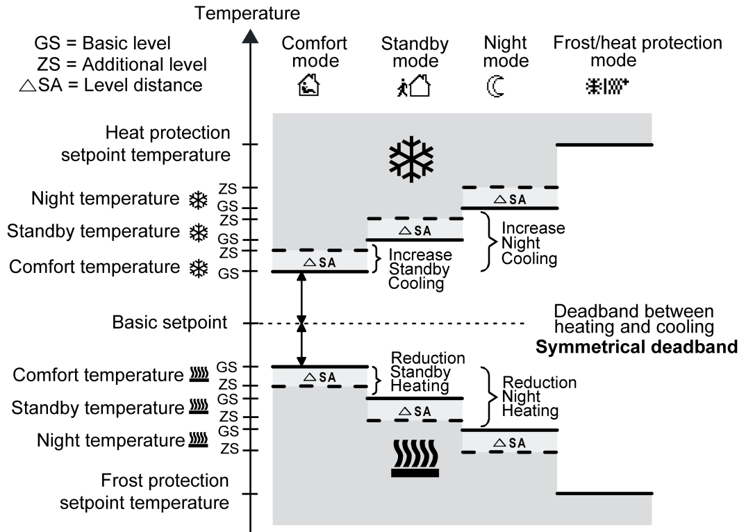
Figure 49: Setpoint temperatures in the operating mode "Basic and additional heating and cooling" with symmetrical deadband
