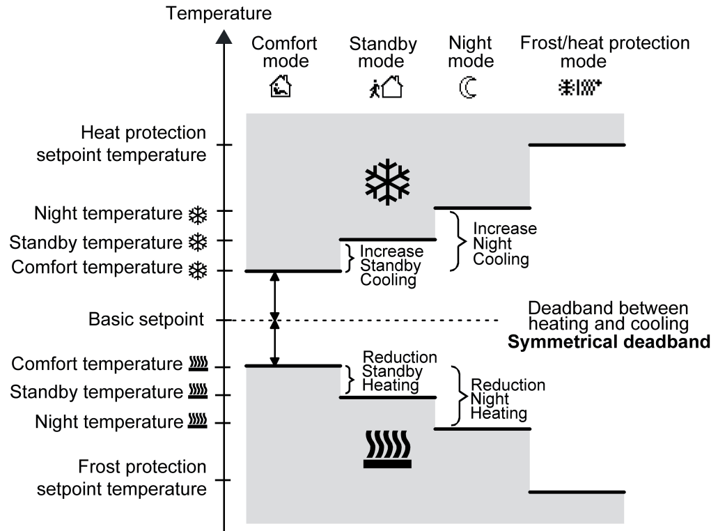
Figure 47: Setpoint temperatures in the operating mode "Heating and cooling" with symmetrical deadband
