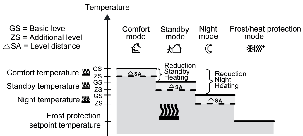
Figure 44: Setpoint temperatures in the operating mode "Basic and additional heating"
