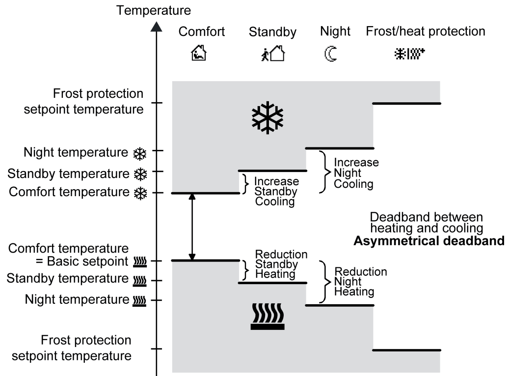
Figure 48: Setpoint temperatures in the operating mode "Heating and cooling" with asymmetrical deadband
