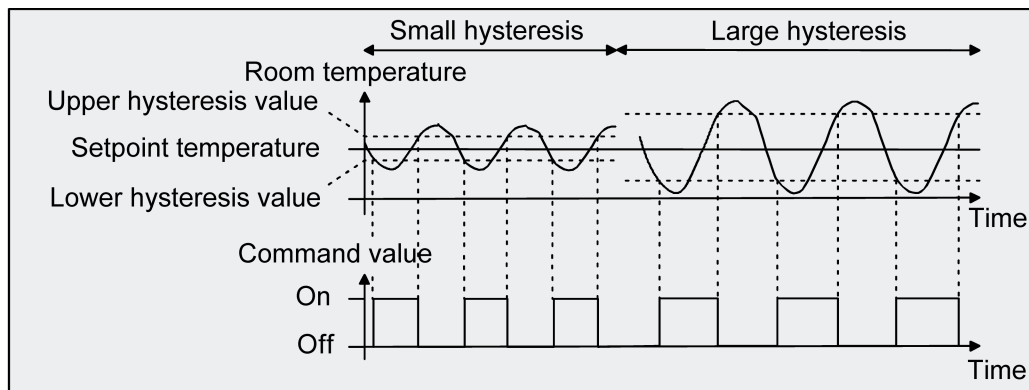
Figure 38: Effects of the hysteresis on the switching behaviour of the command value of 2-point feedback control
