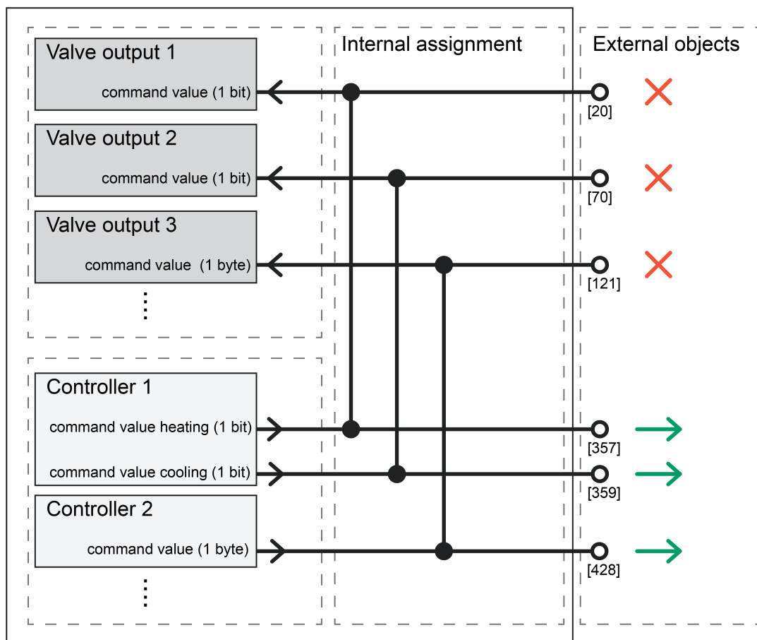
Figure 9: Project design example for internal group communication
