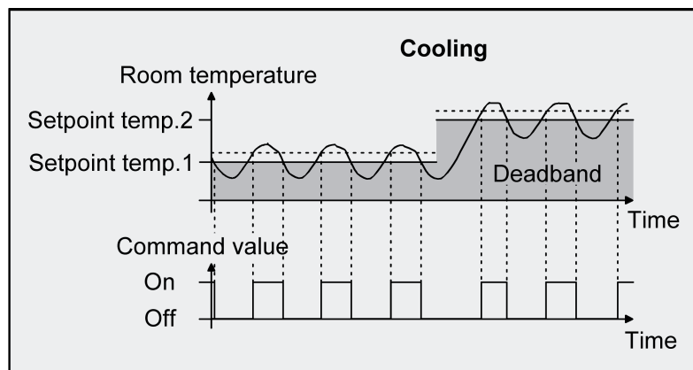
Figure 36: 2-point feedback control for mixed "Heating and cooling" mode with active cooling operation.
