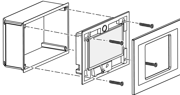
Figure 3: Installation in panel-mounted housing
