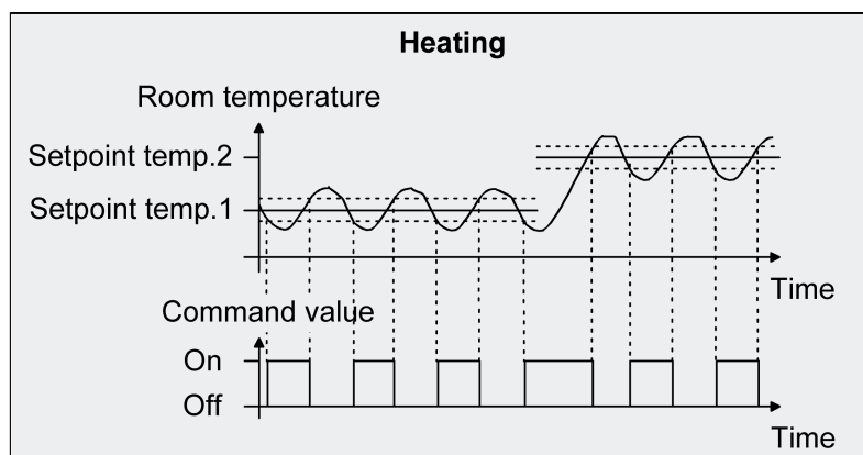
Figure 38: 2-point feedback control for the single "Heating" operating mode
