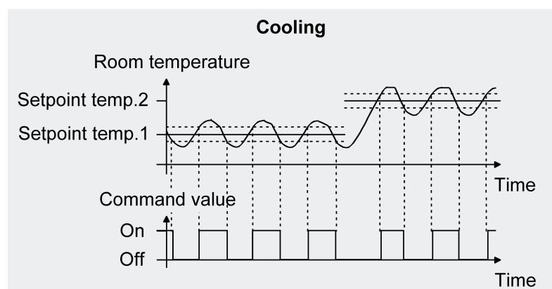
Figure 39: 2-point feedback control for the single "Cooling" operating mode
