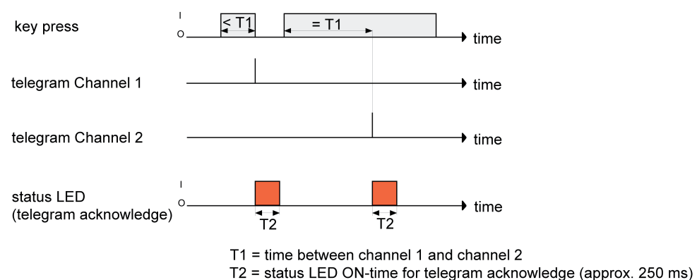
Figure 33: Example of operation concept "Channel 1 or Channel 2"
