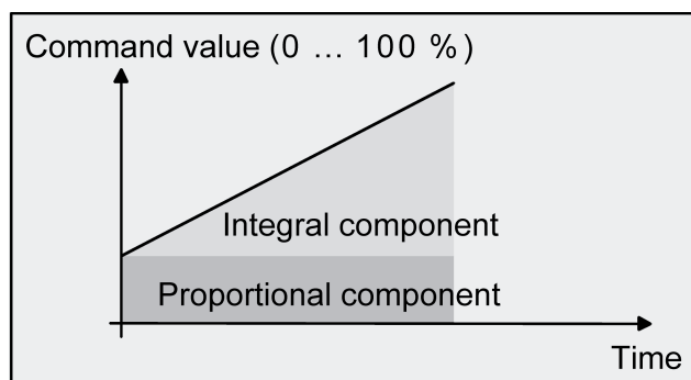
Figure 36: Continuous PI control
