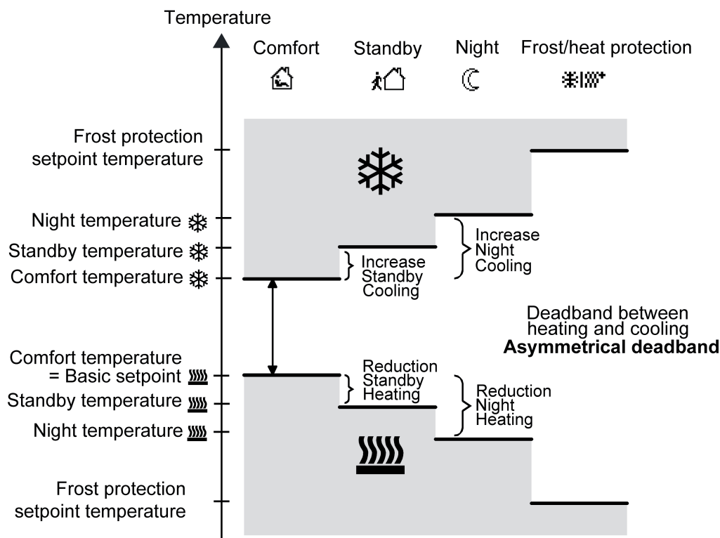
Figure 53: Setpoint temperatures in the operating mode "Heating and cooling" with asymmetrical deadband
