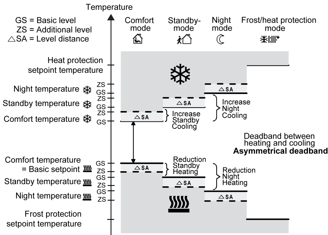
Figure 55: Setpoint temperatures in the operating mode "Basic and additional heating and cooling" with asymmetrical deadband
