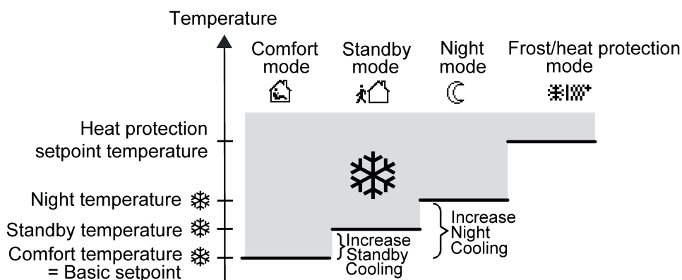
Figure 50: Setpoint temperatures in the operating mode "Cooling"
