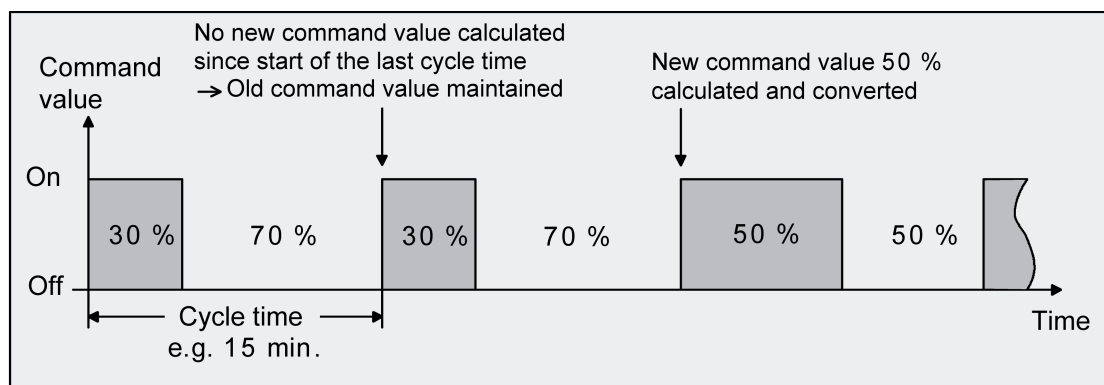
Figure 37: Switching PI control
