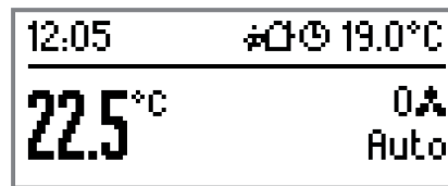
Figure 71: Example for a fan level display in automatic operation
