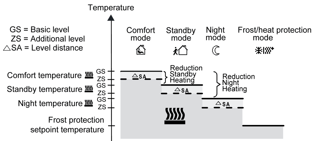
Figure 49: Setpoint temperatures in the operating mode "Basic and additional heating"
