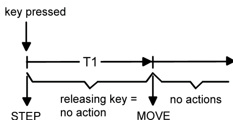
Figure 29: Operation concept "short – long"
