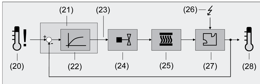
Figure 35: Controlled system of single-room temperature control
