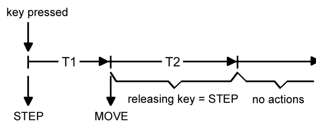
Figure 27: Operation concept "short – long – short"
