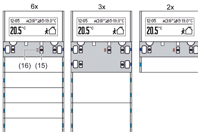
Figure 4: Arrangement of the programming button and LED on the front of the device
