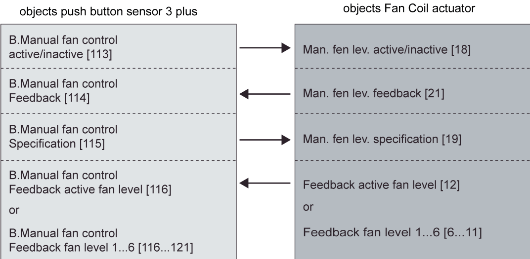
Figure 70: Communication objects of the manual fan control (1-to-1 linking with objects of the fan coil actuator with the same functions)
