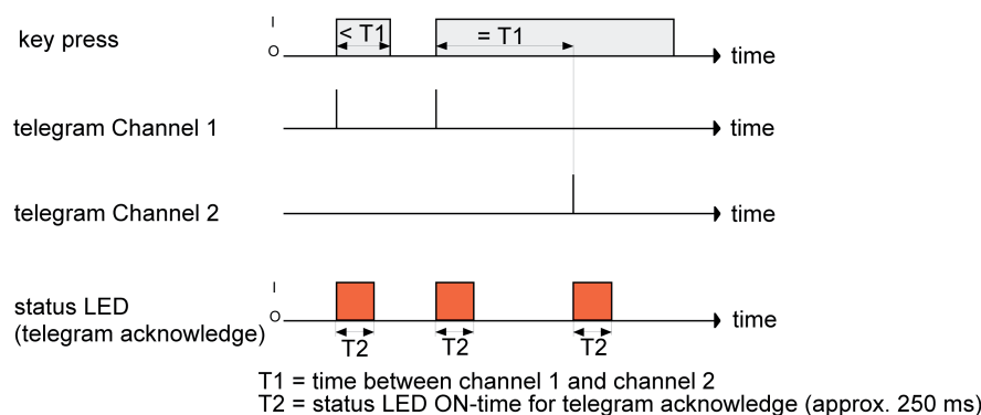
Figure 34: Example for operation concept "Channel 1 and channel 2"
