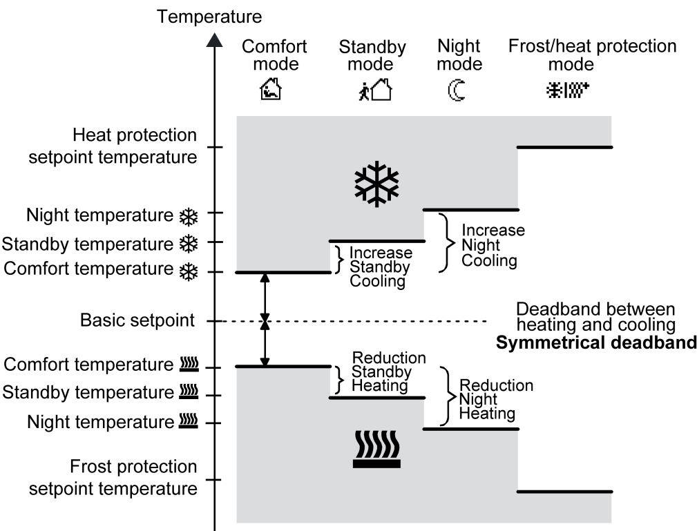
Figure 52: Setpoint temperatures in the operating mode "Heating and cooling" with symmetrical deadband
