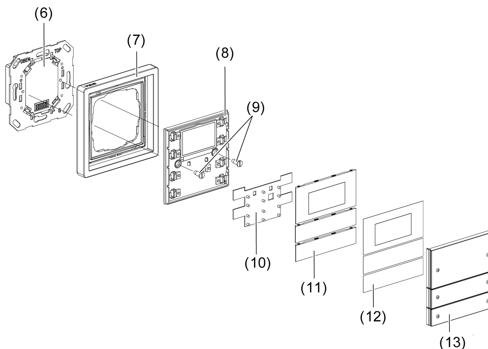
Figure 2: Device fitting of a push button sensor 3 plus 2-gang F100
