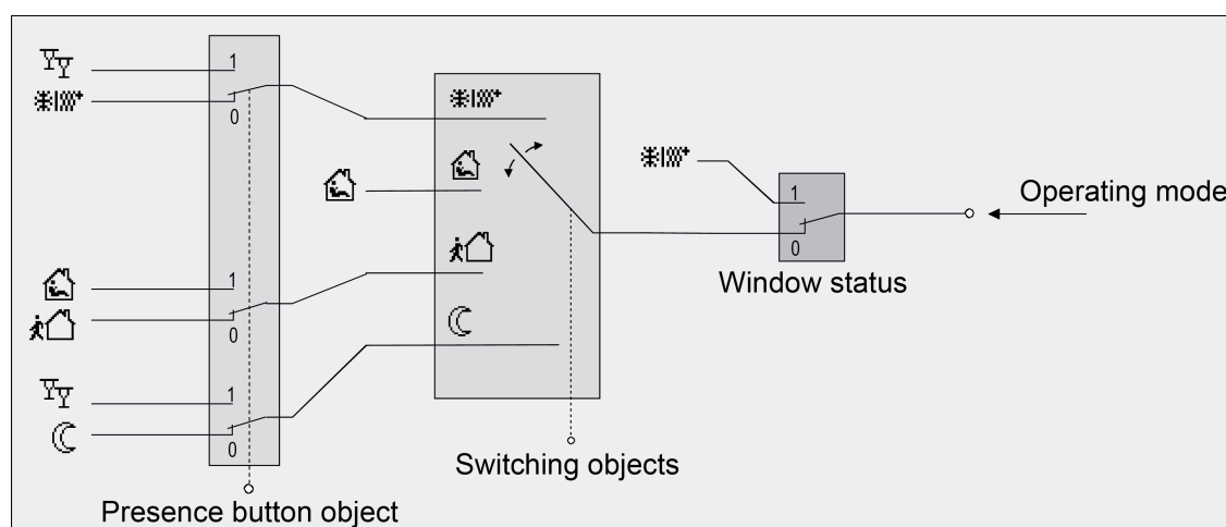
Figure 44: Operating mode change-over through 4 x 1-bit objects with presence button
