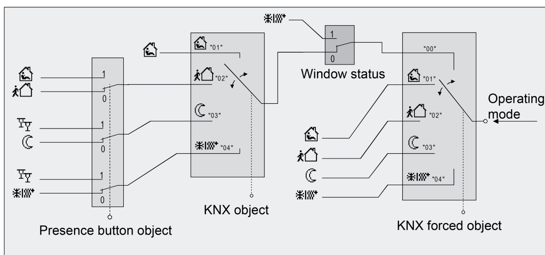
Figure 46: Operating mode change-over through KONNEX object with presence button
