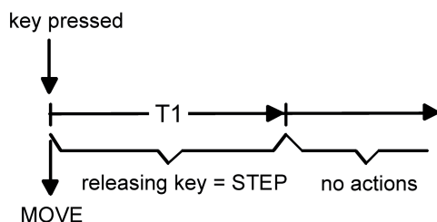
Figure 28: Operation concept "long – short"
