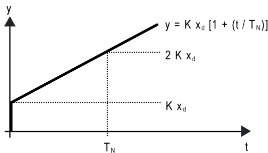
Figure 42: Function of the command value of a PI control
