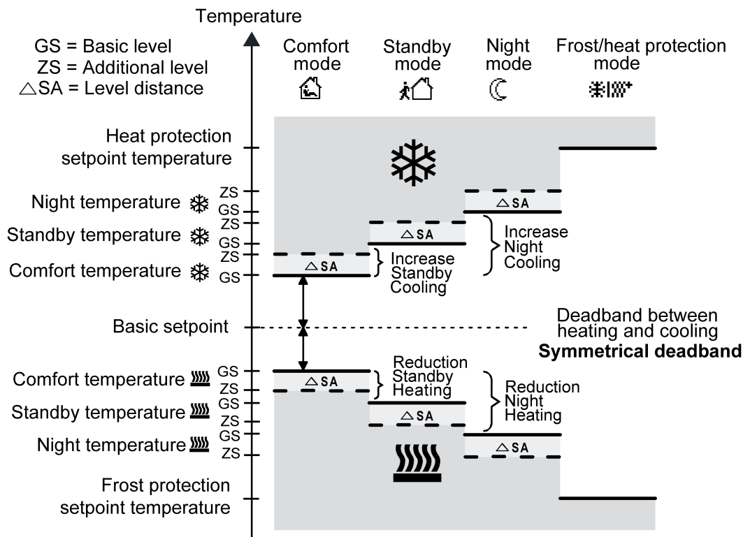
Figure 54: Setpoint temperatures in the operating mode "Basic and additional heating and cooling" with symmetrical deadband
