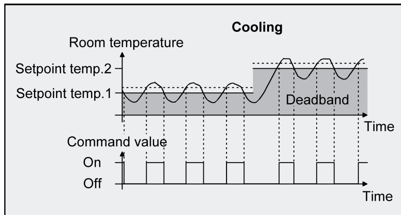
Figure 41: 2-point feedback control for mixed "Heating and cooling" mode with active cooling operation.
