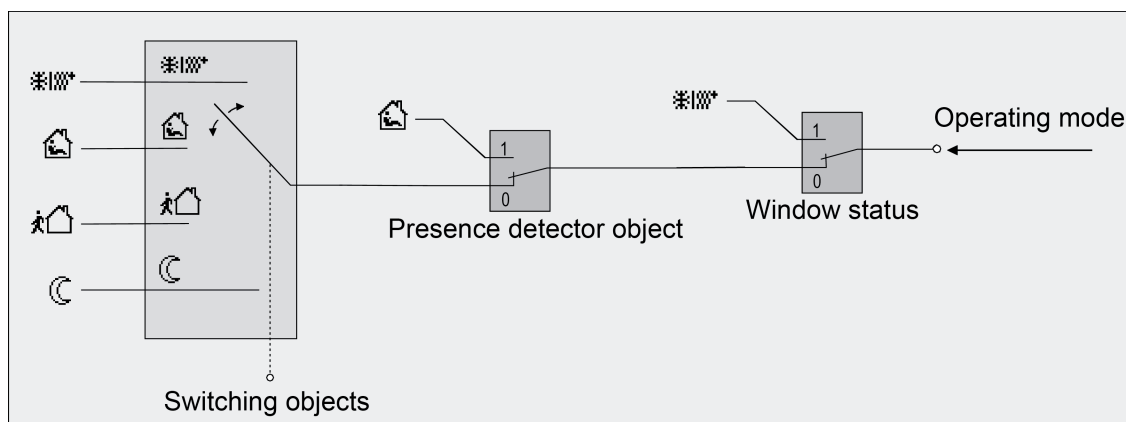
Figure 45: Operating mode change-over through 4 x 1-bit objects with presence detector
