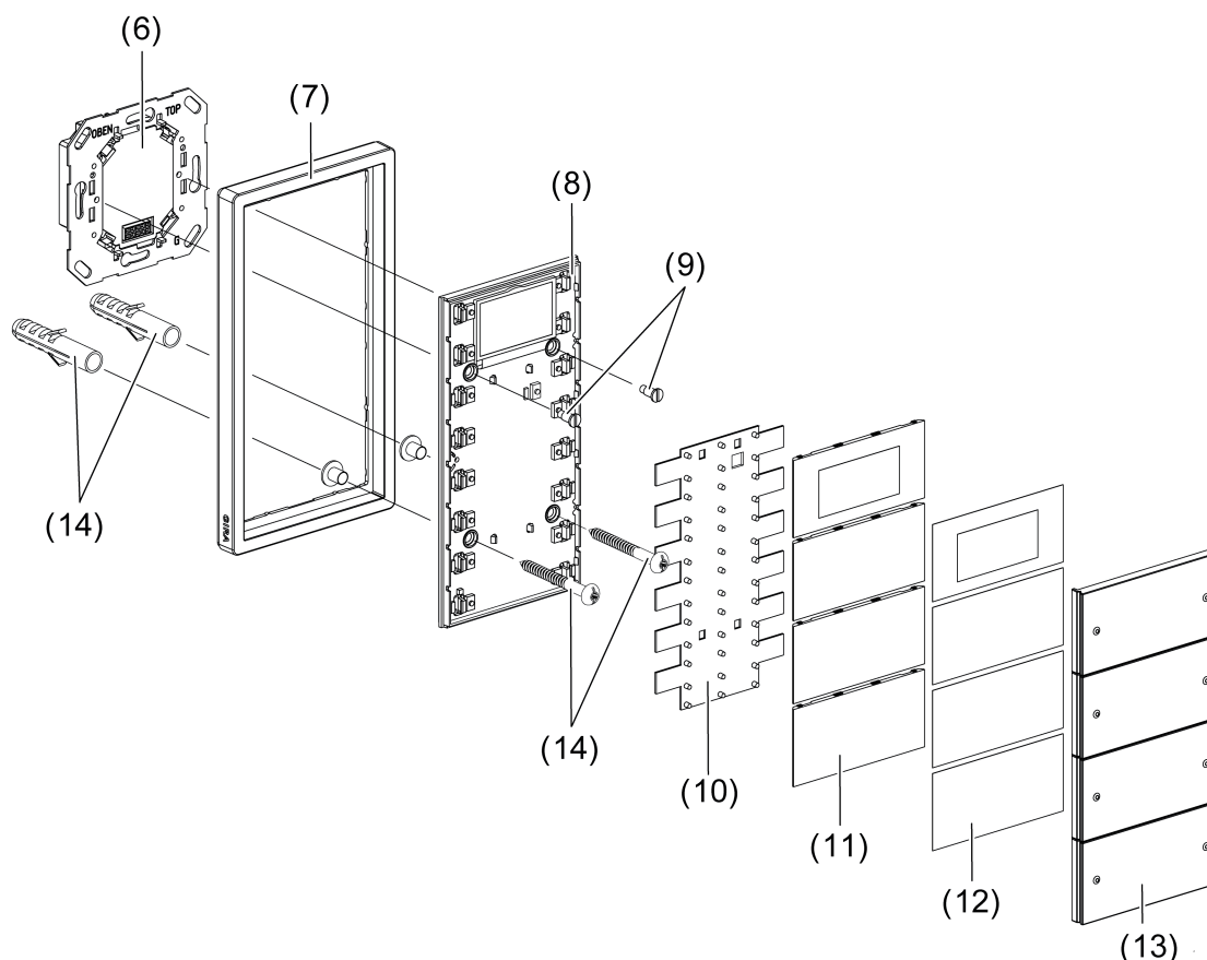
Figure 3: Device fitting using the example of a push button sensor 3 plus 3-gang F100 (doubled height)
