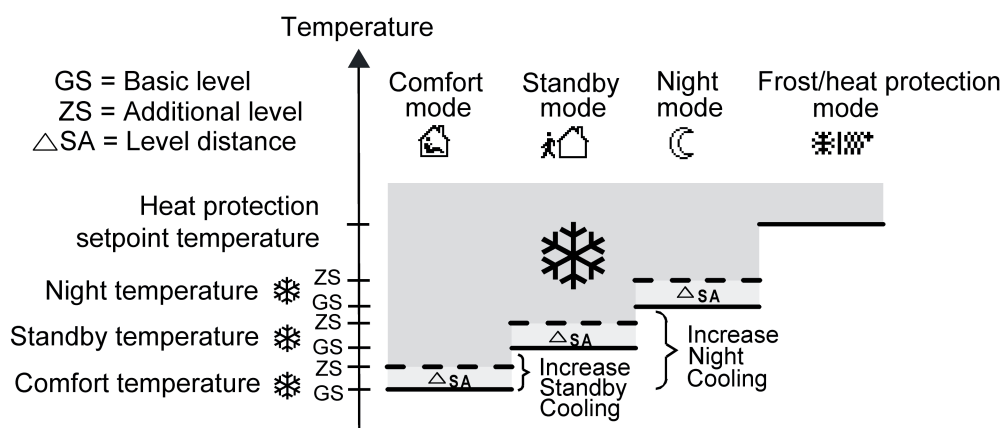
Figure 51: Setpoint temperatures in the operating mode "Basic and additional cooling"
