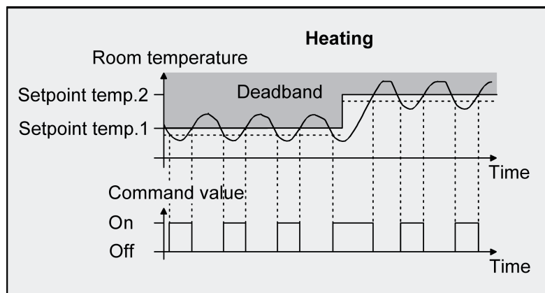
Figure 40: 2-point feedback control for mixed "Heating and cooling" mode with active heating mode.
