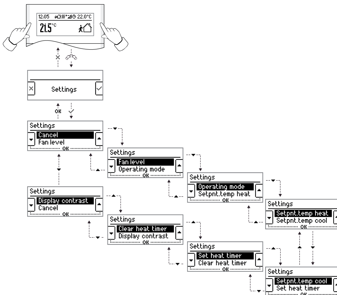
Figure 9: Navigation through the main menu of the device settings
