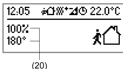
Figure 60: Example of a 2-area display with 2-line value display Line 1 brightness value, line 2 slat angle
