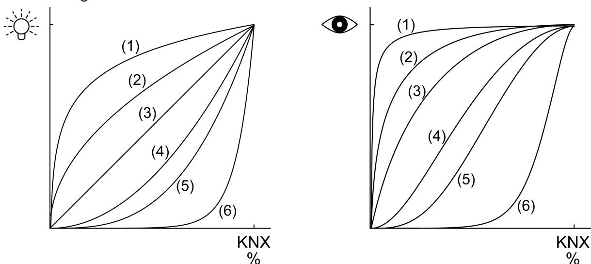
Figure 6: Dimming characteristics in the value range
