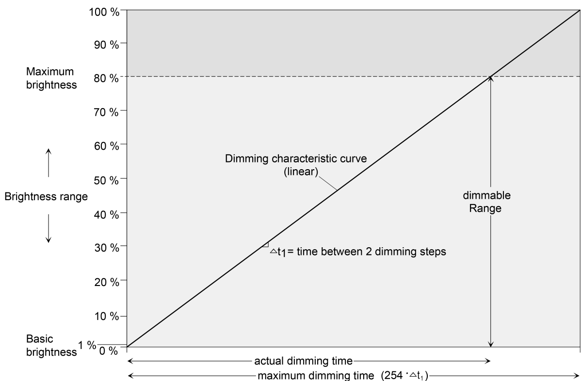
Figure 7: Linear dimming characteristic as an example with basic brightness and maximum brightness
