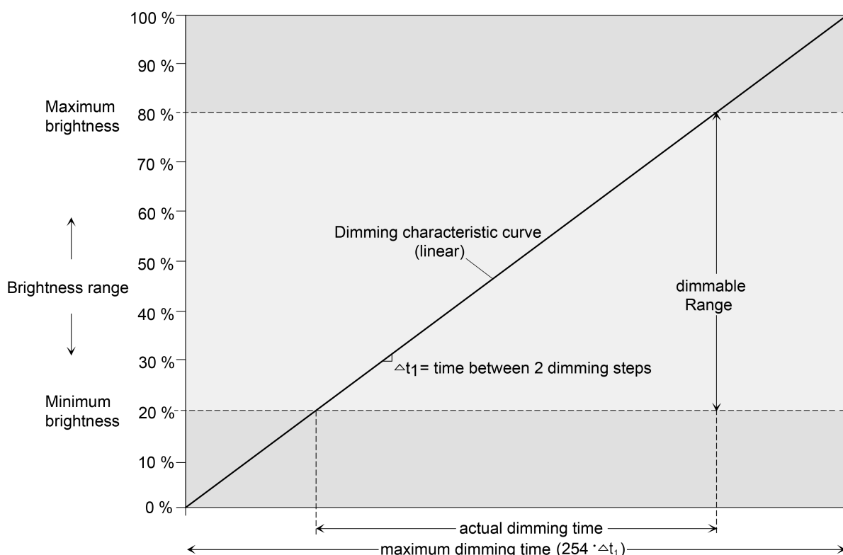
Figure 8: Linear characteristic dimming curve as an example with minimum brightness > 0 % and maximum brightness
