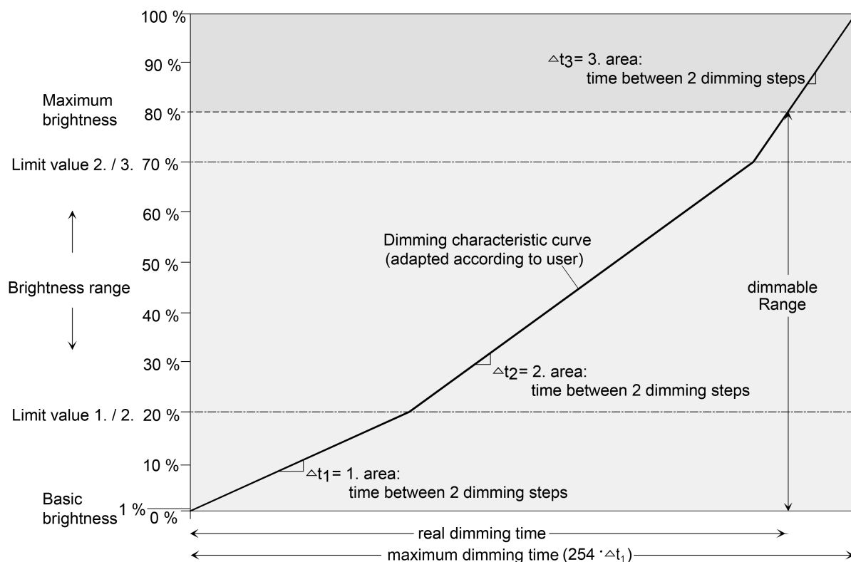
Figure 9: User-defined dimming characteristic as an example with basic brightness and maximum brightness
