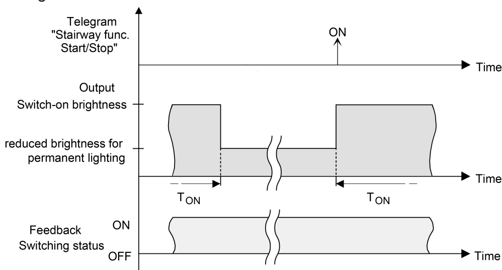
Figure 22: The continuous lighting of the staircase function without soft functions
