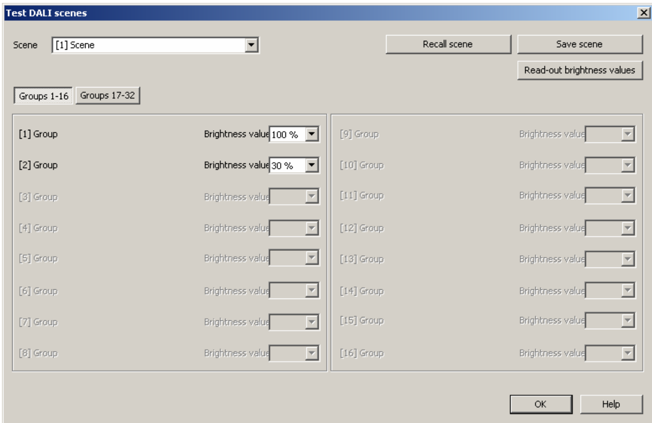
Figure 50: Scene-oriented DALI test environment (in this example with two created groups)
