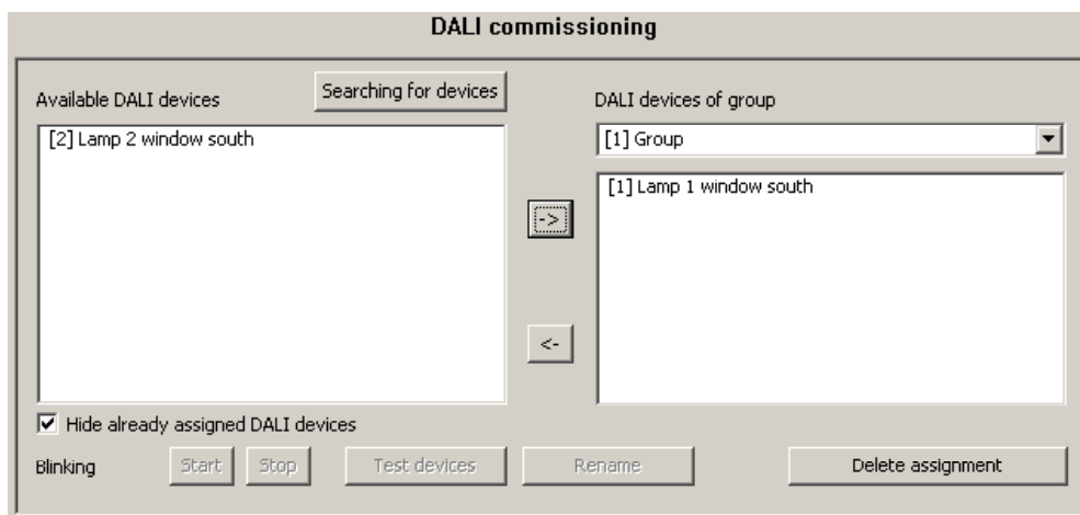
Fig 41: Assigning a device to a group
