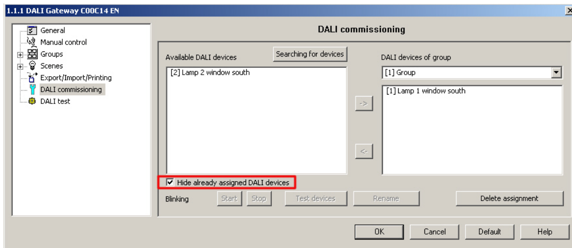
Figure 39: Check box "Hide already assigned DALI devices" in the DALI commissioning dialog of the ETS plug-in
