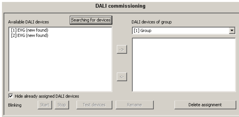
Figure 37: An example of the device list after a search (the example shows two newly identified electronic ballast devices)
