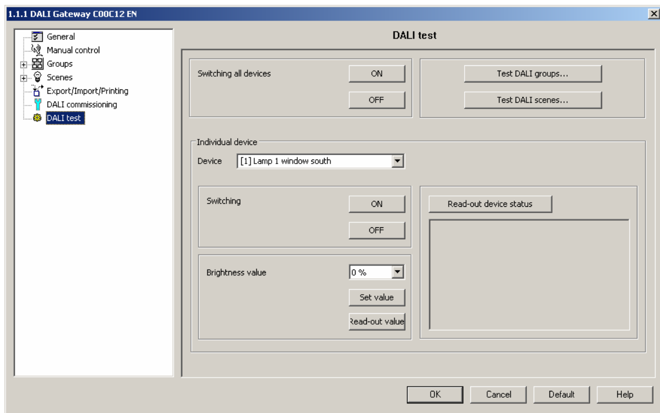
Figure 46: DALI test environment in the ETS 3 plug-in
